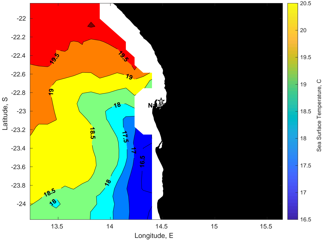
SST for Nautilus at 08-Mar-2025 00:00:00
