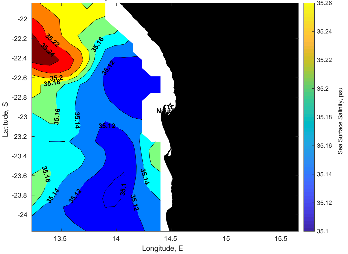
Surface Salinity for Nautilus at 08-Mar-2025 00:00:00
