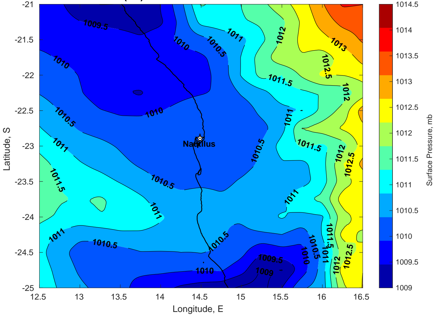
Surface Pressure (mb) for Nautilus at 09-Mar-2025 00:00:00
