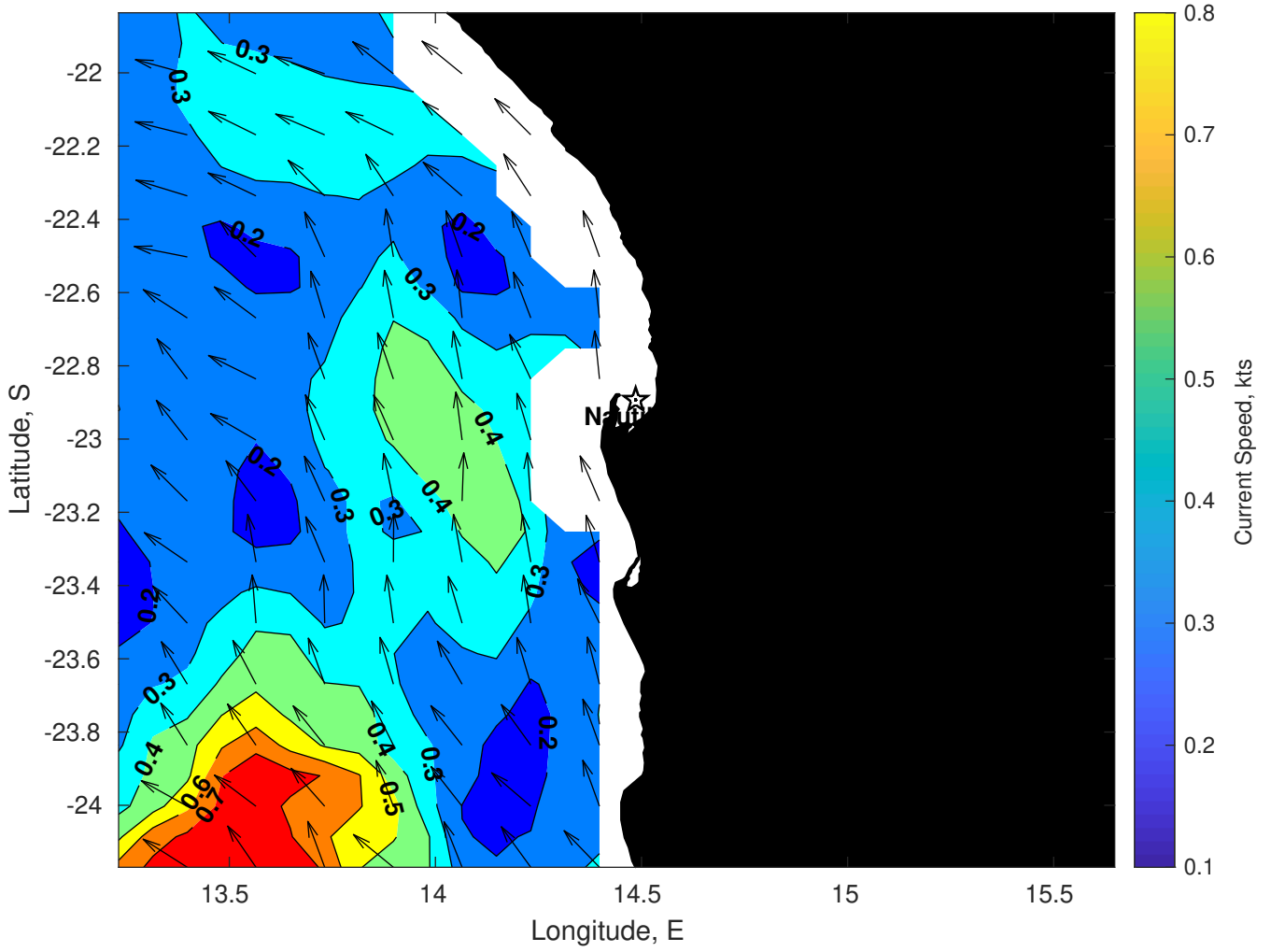
Surface Currents for Nautilus at 08-Mar-2025 00:00:00
