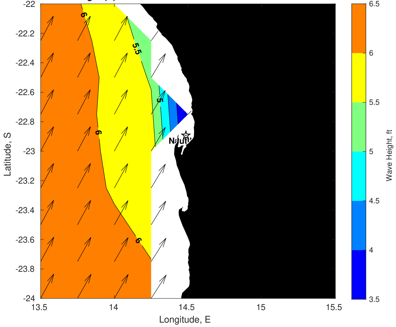
Wave Height (ft) for Nautilus at 09-Mar-2025 09:00:00
