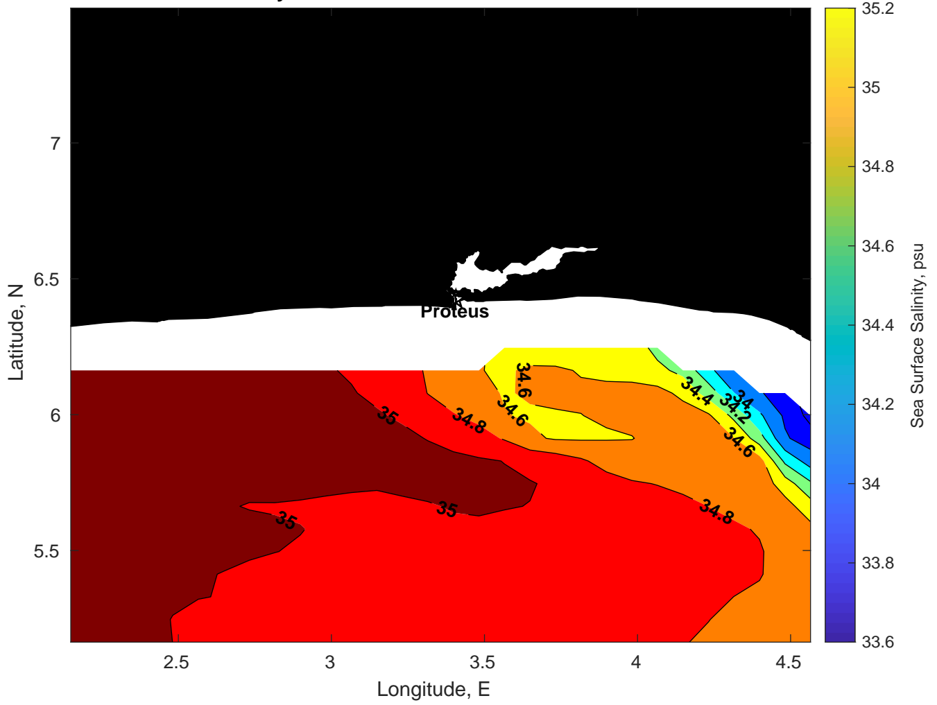
Surface Salinity for Proteus at 08-Mar-2025 00:00:00
