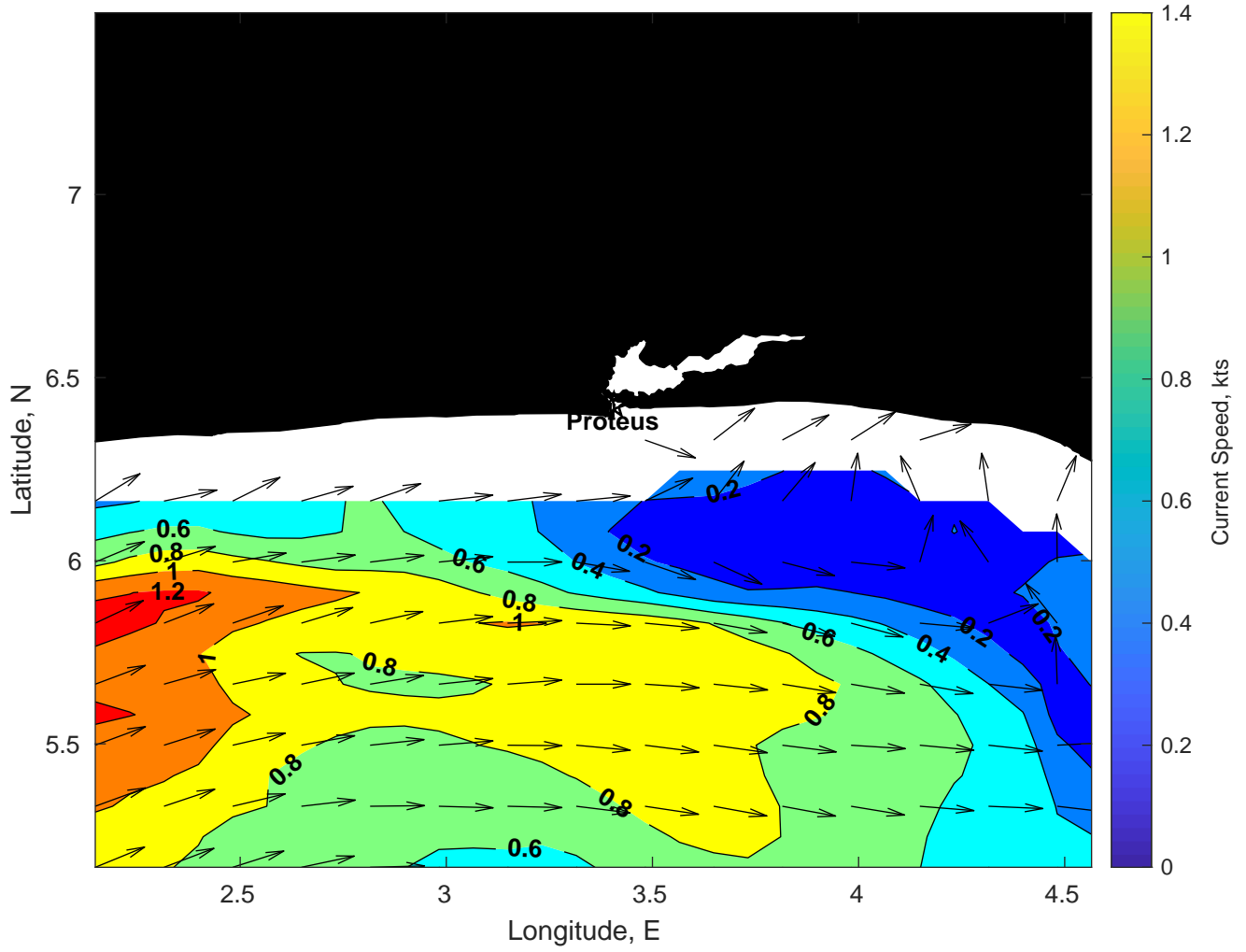
Surface Currents for Proteus at 08-Mar-2025 00:00:00
