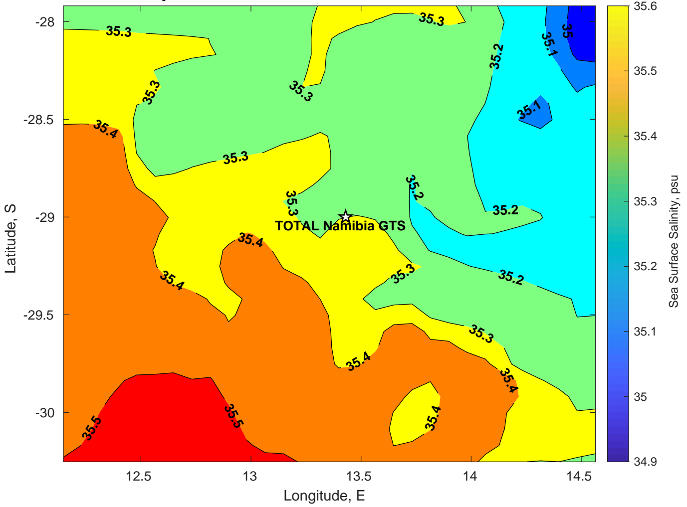
Surface Salinity for TOTAL Namibia GTS at 08-Mar-2025 00:00:00
