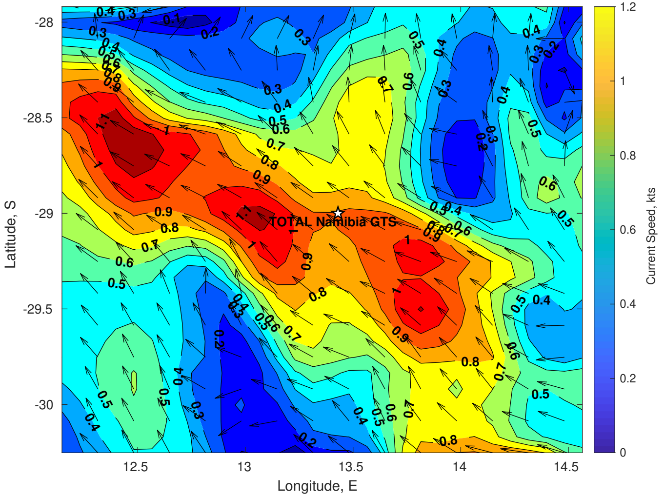
Surface Currents for TOTAL Namibia GTS at 08-Mar-2025 00:00:00
