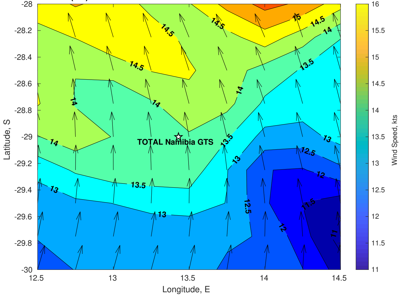
Winds (kts) for TOTAL Namibia GTS at 09-Mar-2025 09:00:00
