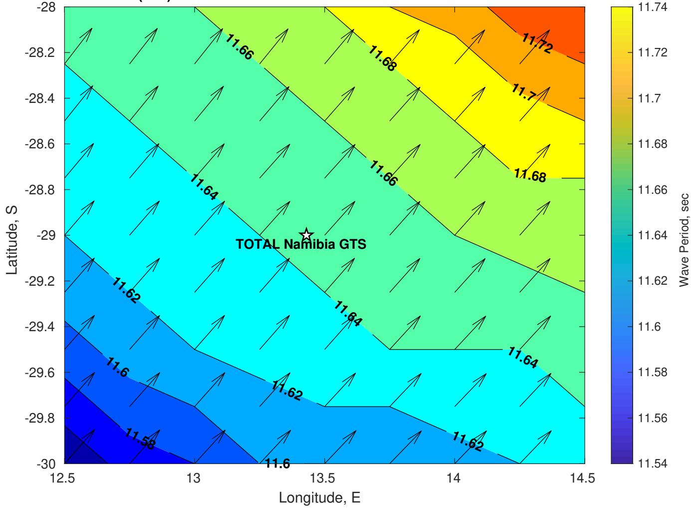
Wave Period (sec) for TOTAL Namibia GTS at 09-Mar-2025 09:00:00
