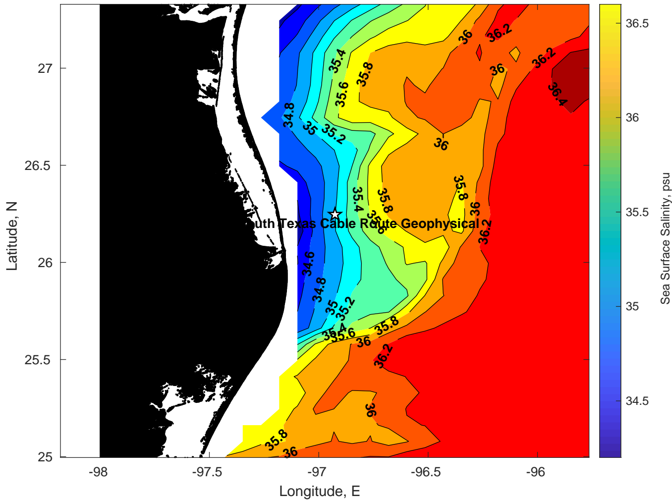
Surface Salinity for Tampnet P2378 South Texas Cable Route Geophysical at 08-Mar-2025 00:00:00
