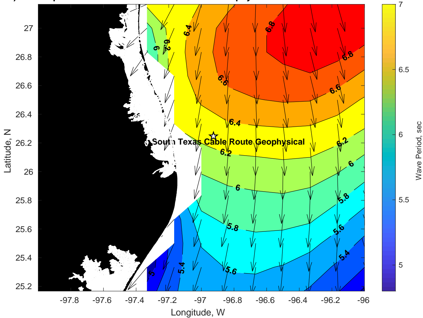
Period (sec) for Tampnet P2378 South Texas Cable Route Geophysical at 09-Mar-2025 09:00:00
