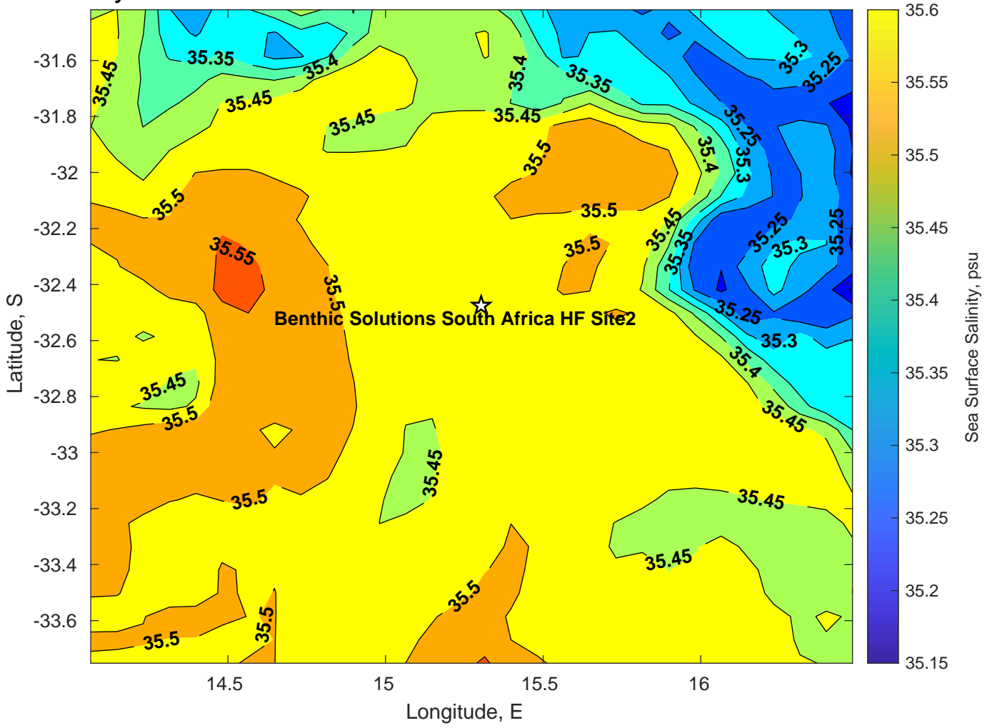
Surface Salinity for Benthic Solutions South Africa HF Site2 at 09-Mar-2025 00:00:00
