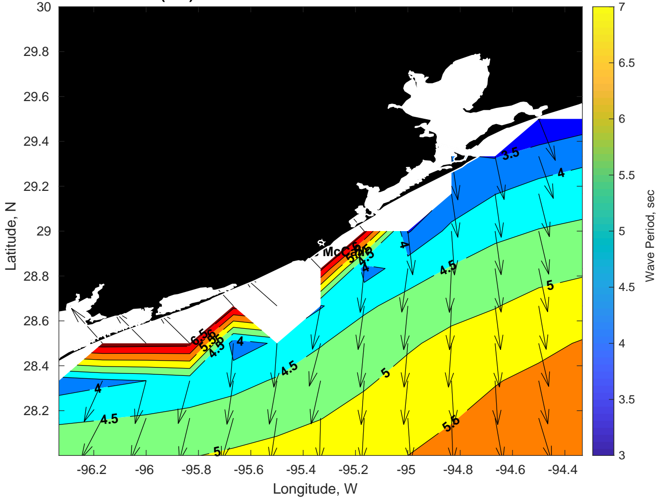
Wave Period (sec) for Brooks McCall at 10-Mar-2025 09:00:00
