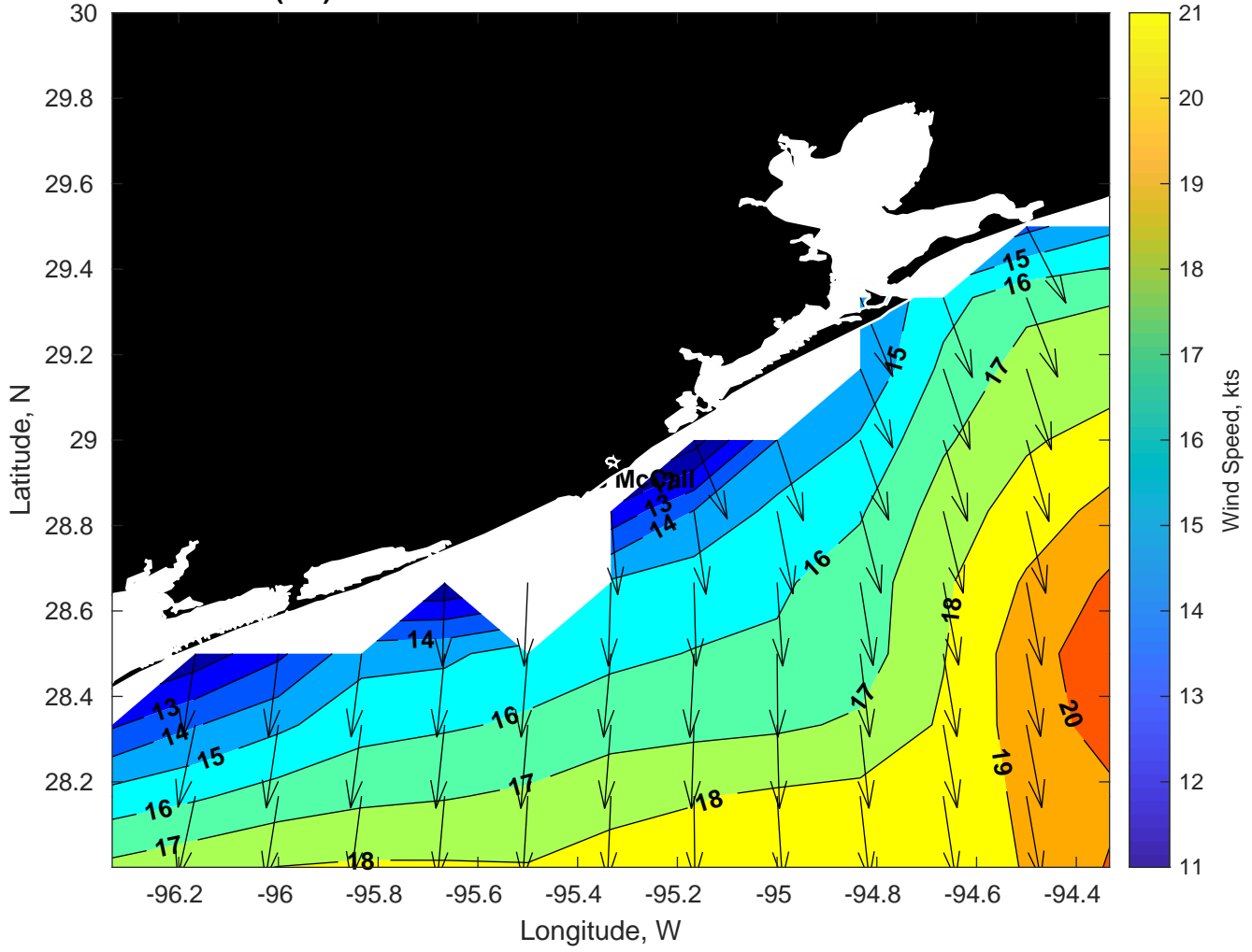
Winds (kts) for Brooks McCall at 10-Mar-2025 09:00:00
