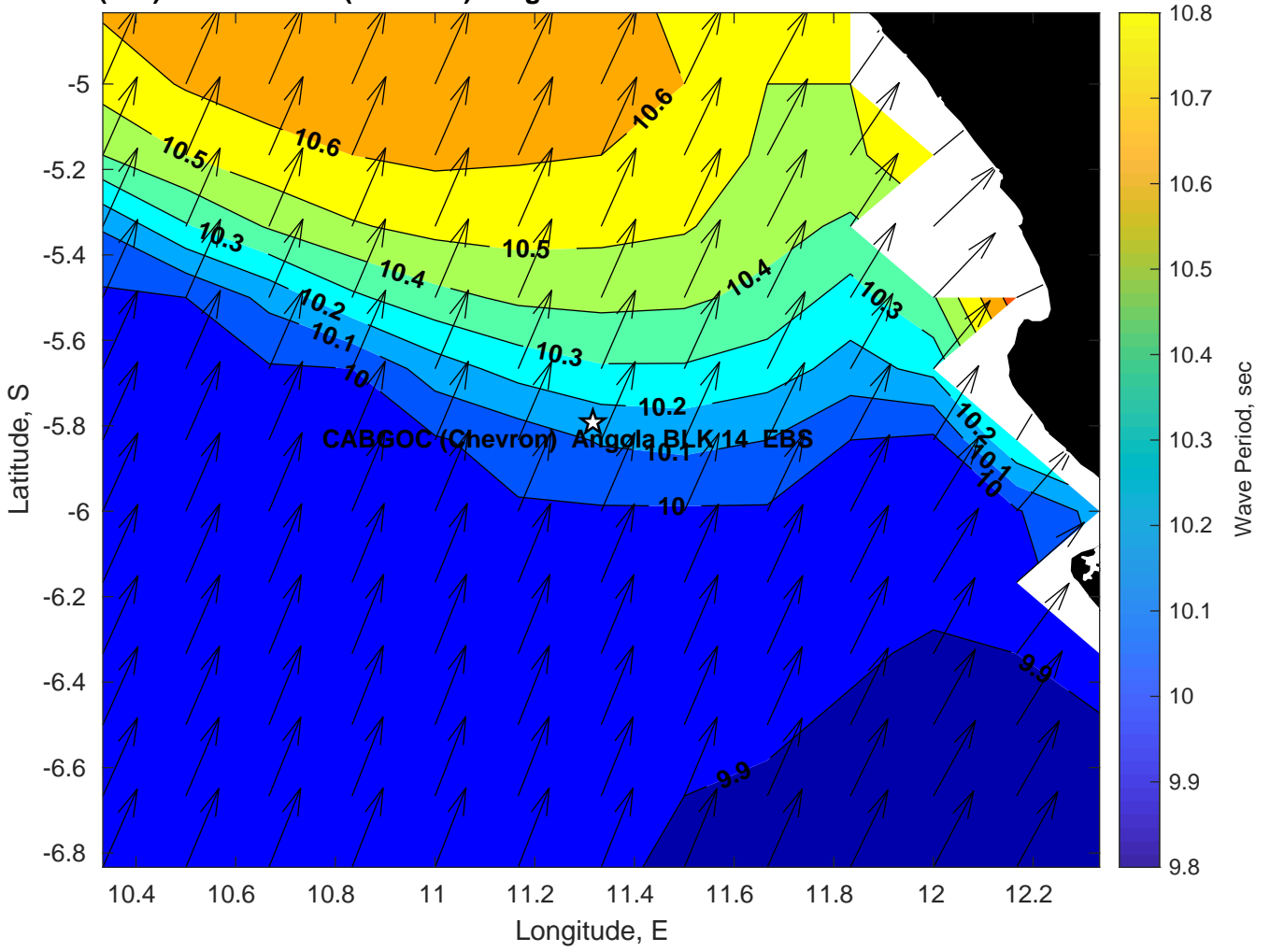
Wave Period (sec) for CABGOC (Chevron) Angola BLK 14 EBS at 10-Mar-2025 09:00:00
