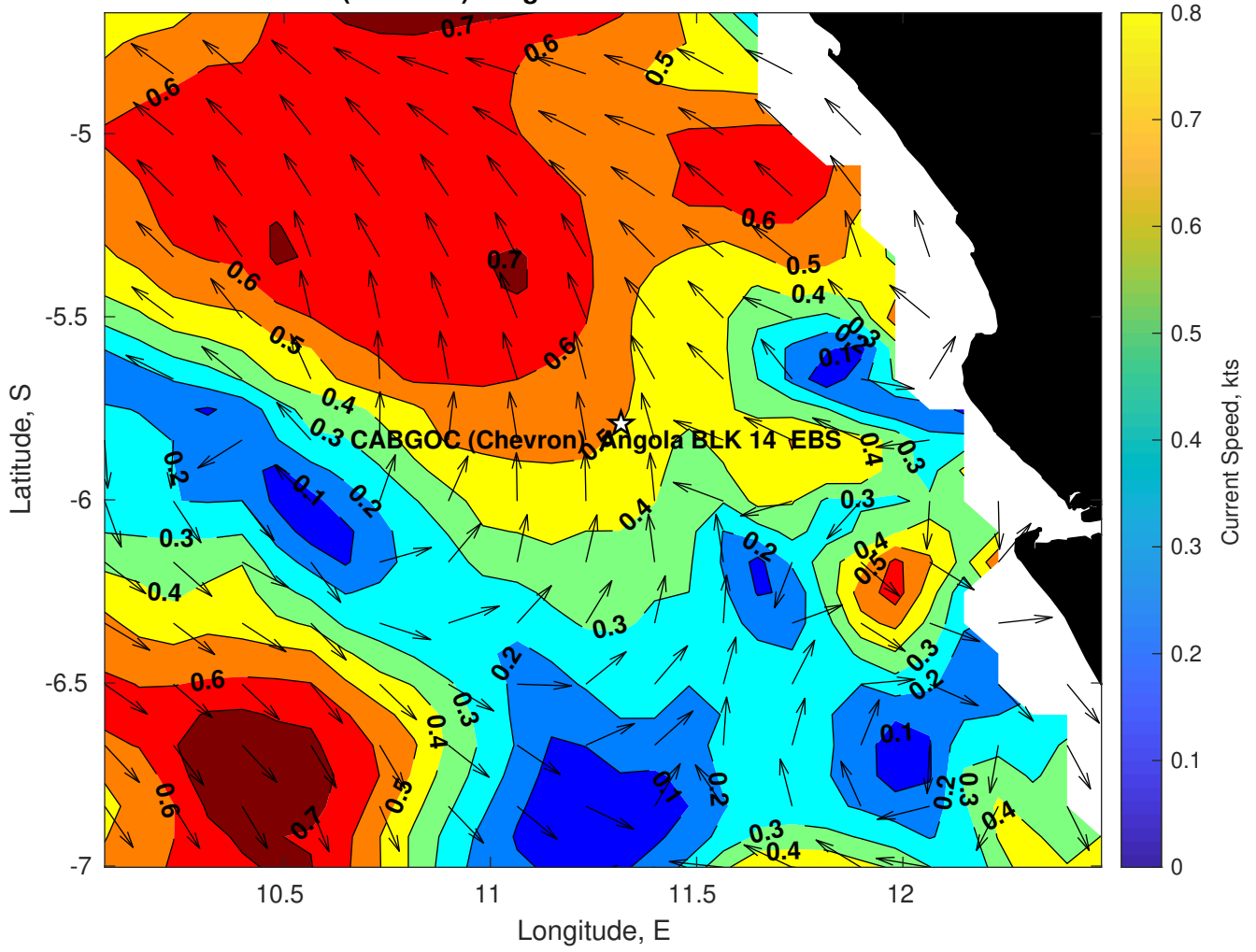
Surface Currents for CABGOC (Chevron) Angola BLK 14 EBS at 09-Mar-2025 00:00:00
