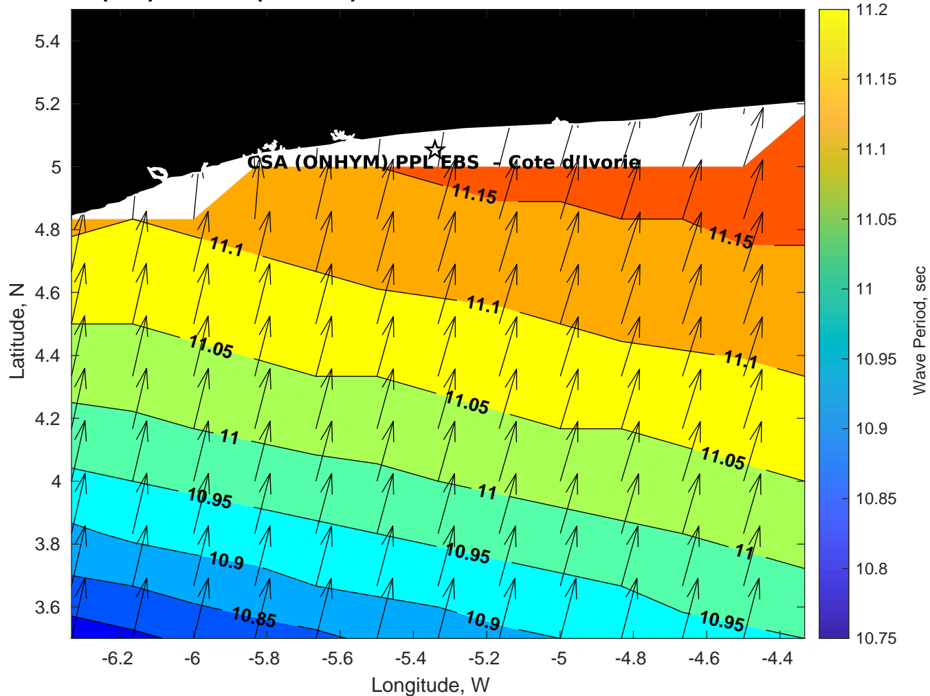
Wave Period (sec) for CSA (ONHYM) PPL EBS - Cote d'Ivoire at 10-Mar-2025 09:00:00
