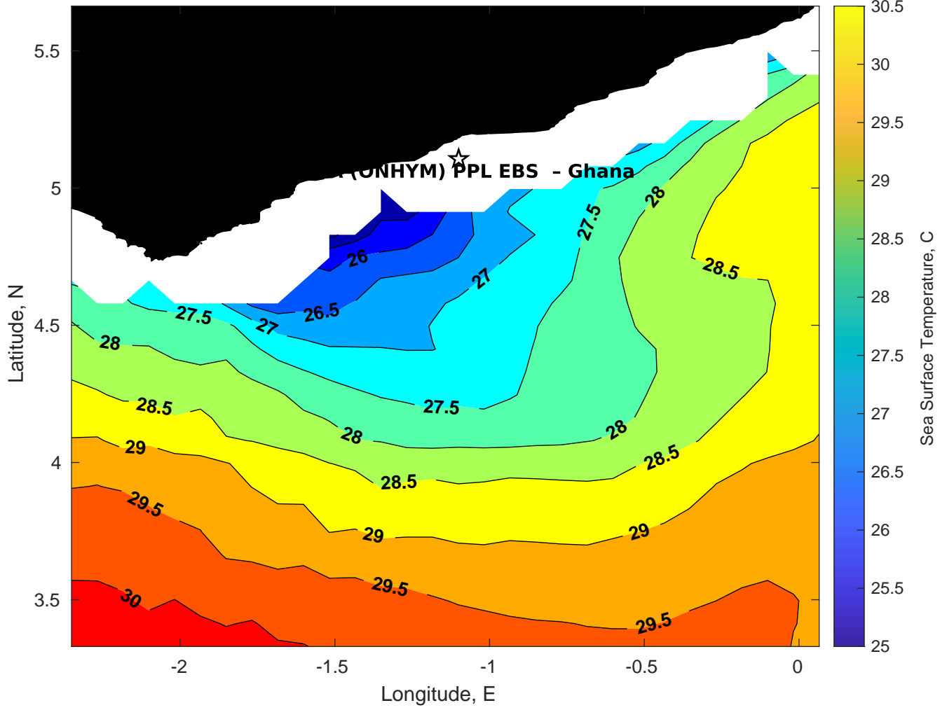
SST for CSA (ONHYM) PPL EBS - Ghana at 09-Mar-2025 00:00:00
