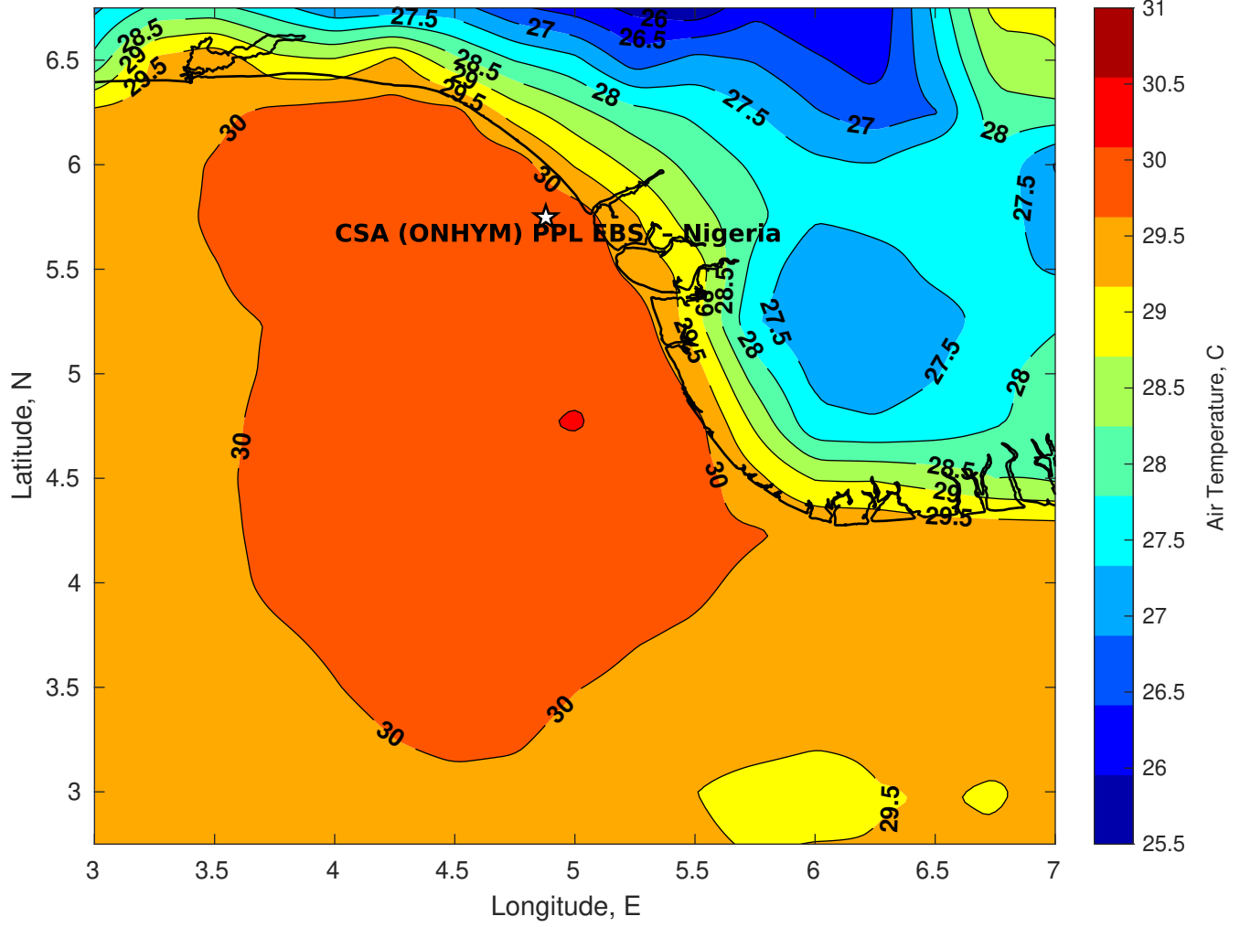
Air Temperature (C) for CSA (ONHYM) PPL EBS - Nigeria at 10-Mar-2025
