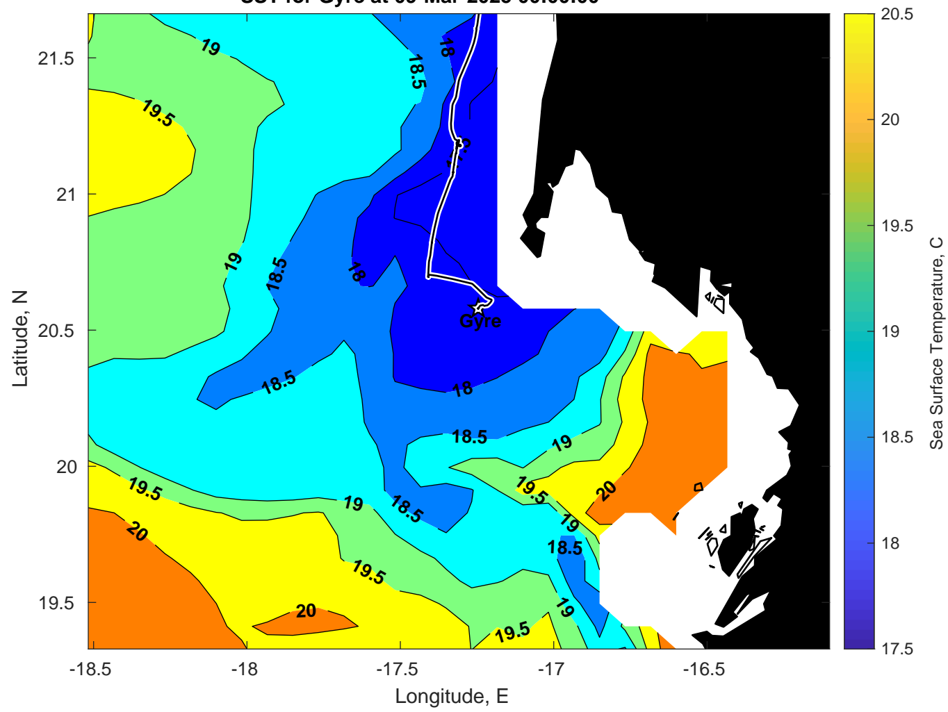
SST for Gyre at 09-Mar-2025 00:00:00
