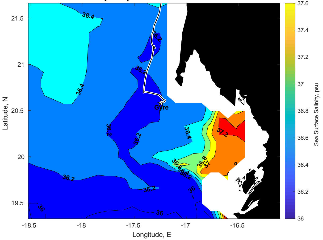
Surface Salinity for Gyre at 09-Mar-2025 00:00:00
