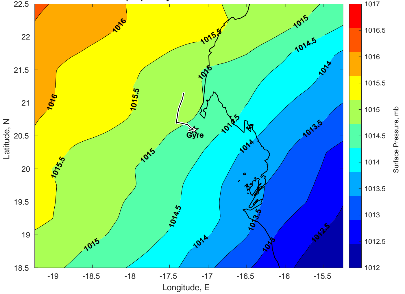
Surface Pressure (mb) for Gyre at 10-Mar-2025 00:00:00
