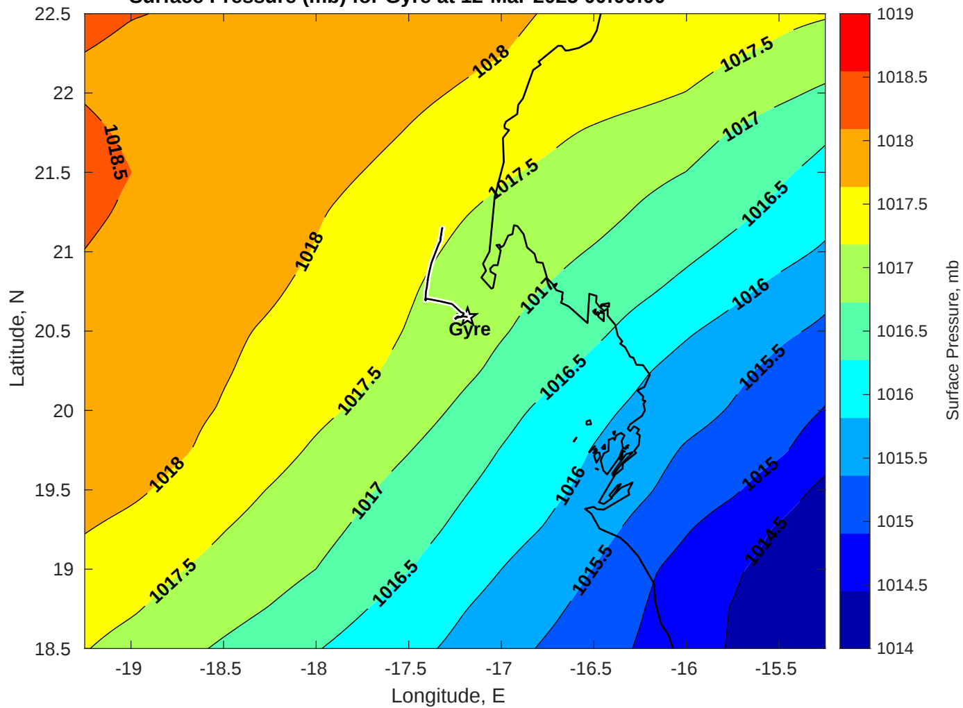
Surface Pressure (mb) for Gyre at 12-Mar-2025 00:00:00
