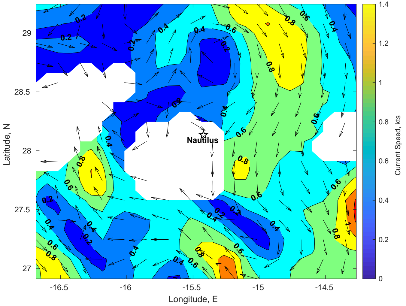
Surface Currents for Nautilus at 09-Mar-2025 00:00:00
