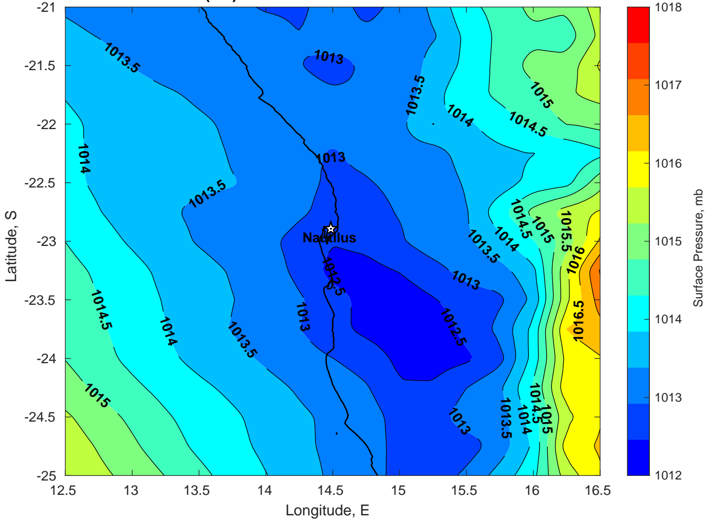
Surface Pressure (mb) for Nautilus at 10-Mar-2025 00:00:00
