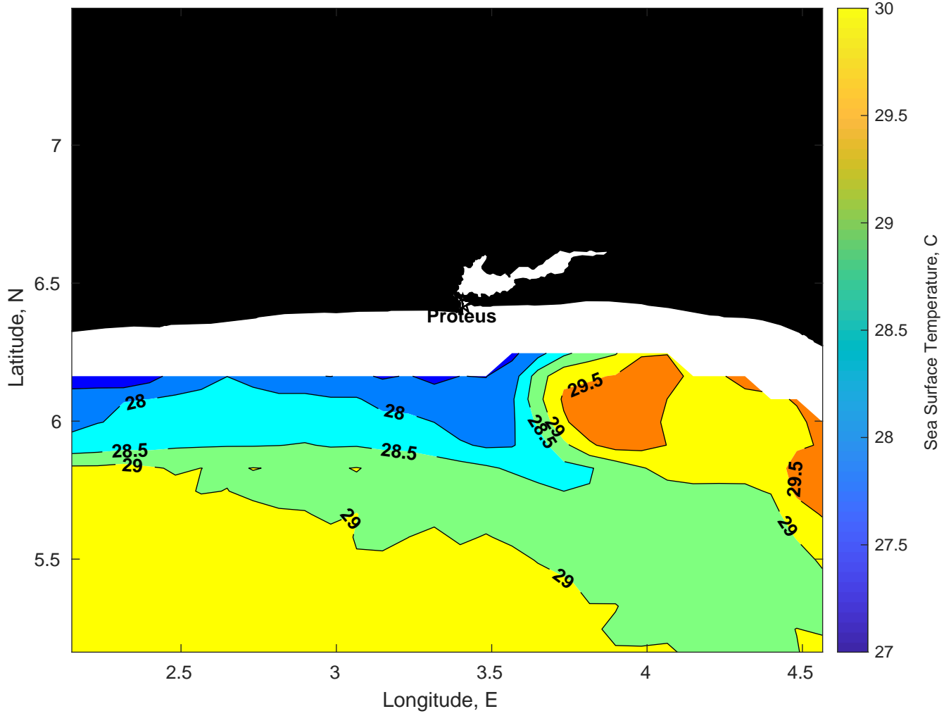
SST for Proteus at 09-Mar-2025 00:00:00
