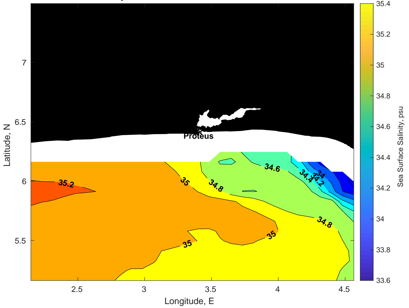
Surface Salinity for Proteus at 09-Mar-2025 00:00:00
