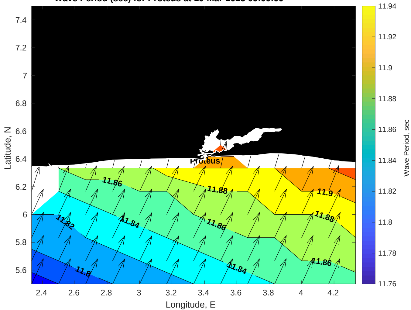
Wave Period (sec) for Proteus at 10-Mar-2025 09:00:00
