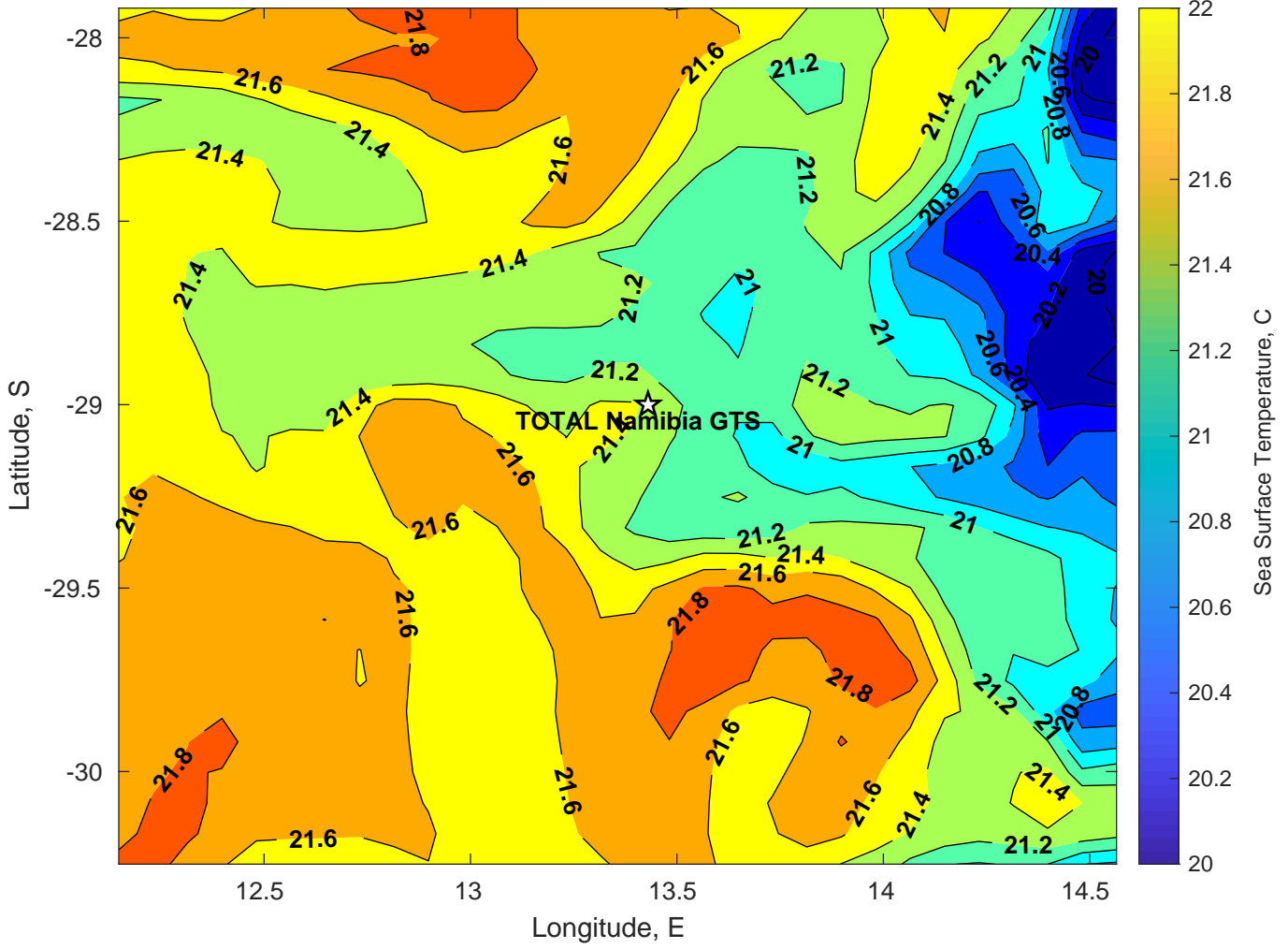
SST for TOTAL Namibia GTS at 09-Mar-2025 00:00:00
