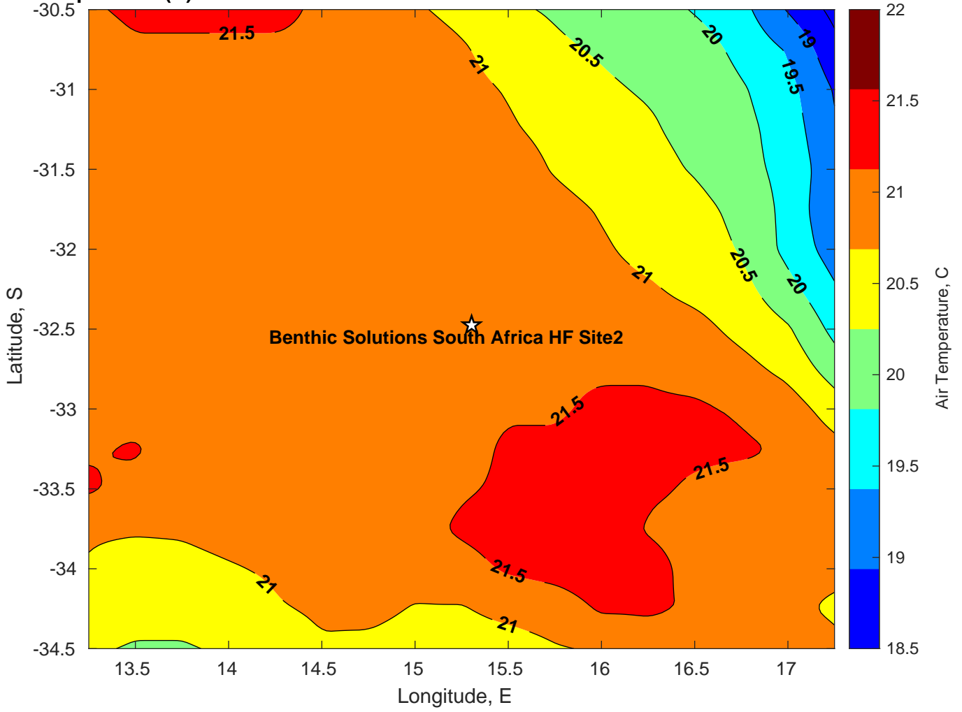
Air Temperature (C) for Benthic Solutions South Africa HF Site2 at 11-Mar-2025
