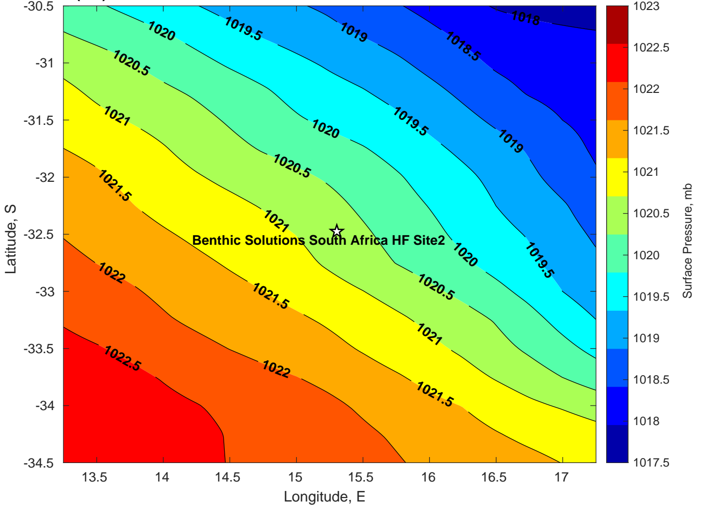
Surface Pressure (mb) for Benthic Solutions South Africa HF Site2 at 11-Mar-2025 00:00:00
