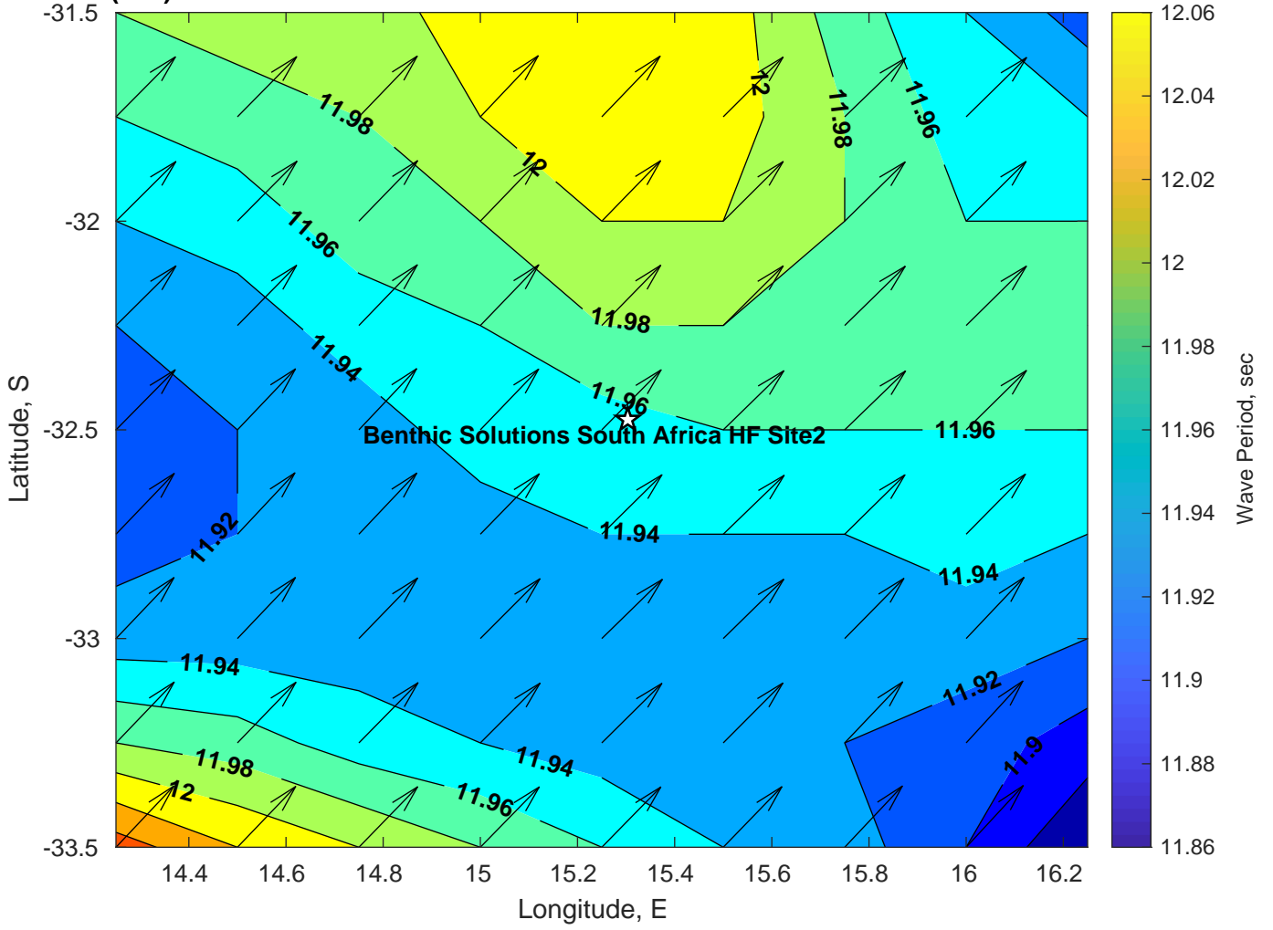
Wave Period (sec) for Benthic Solutions South Africa HF Site2 at 11-Mar-2025 09:00:00
