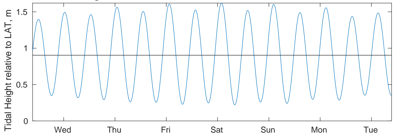
Tidal Currents and Heights for Benthic Solutions South Africa HF Site2 at 20250311
