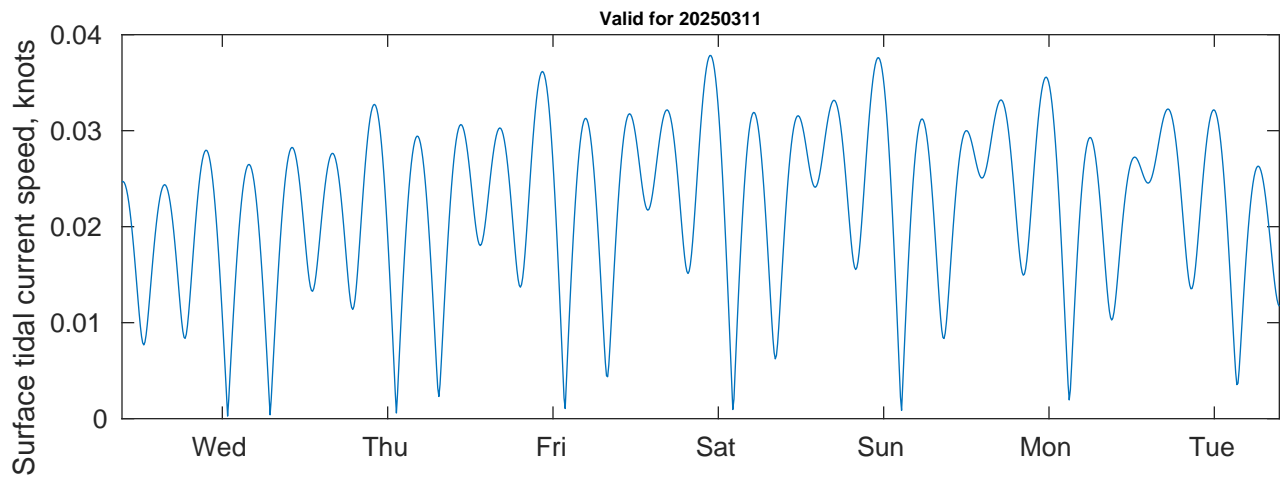
Tidal Currents and Heights for Benthic Solutions South Africa HF Site2 at 20250311
