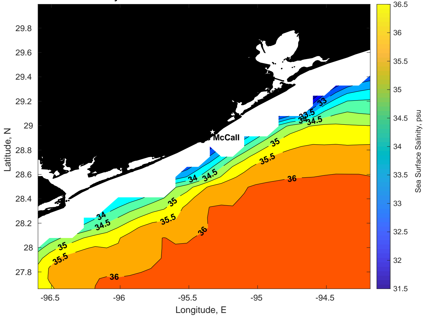
Surface Salinity for Brooks McCall at 10-Mar-2025 00:00:00
