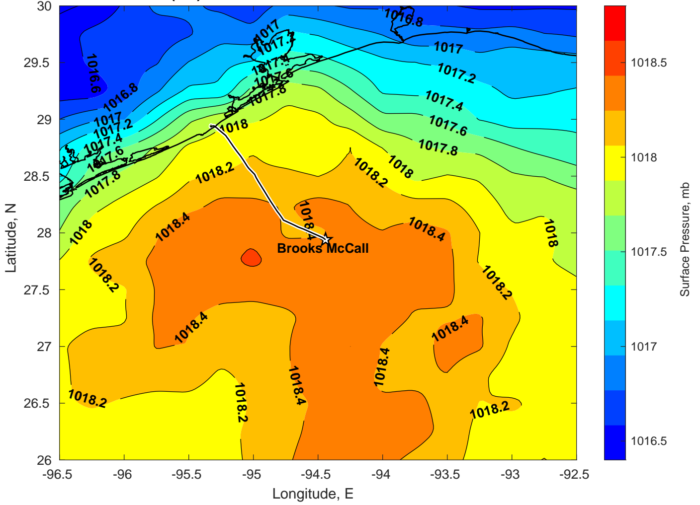
Surface Pressure (mb) for Brooks McCall at 11-Mar-2025 00:00:00
