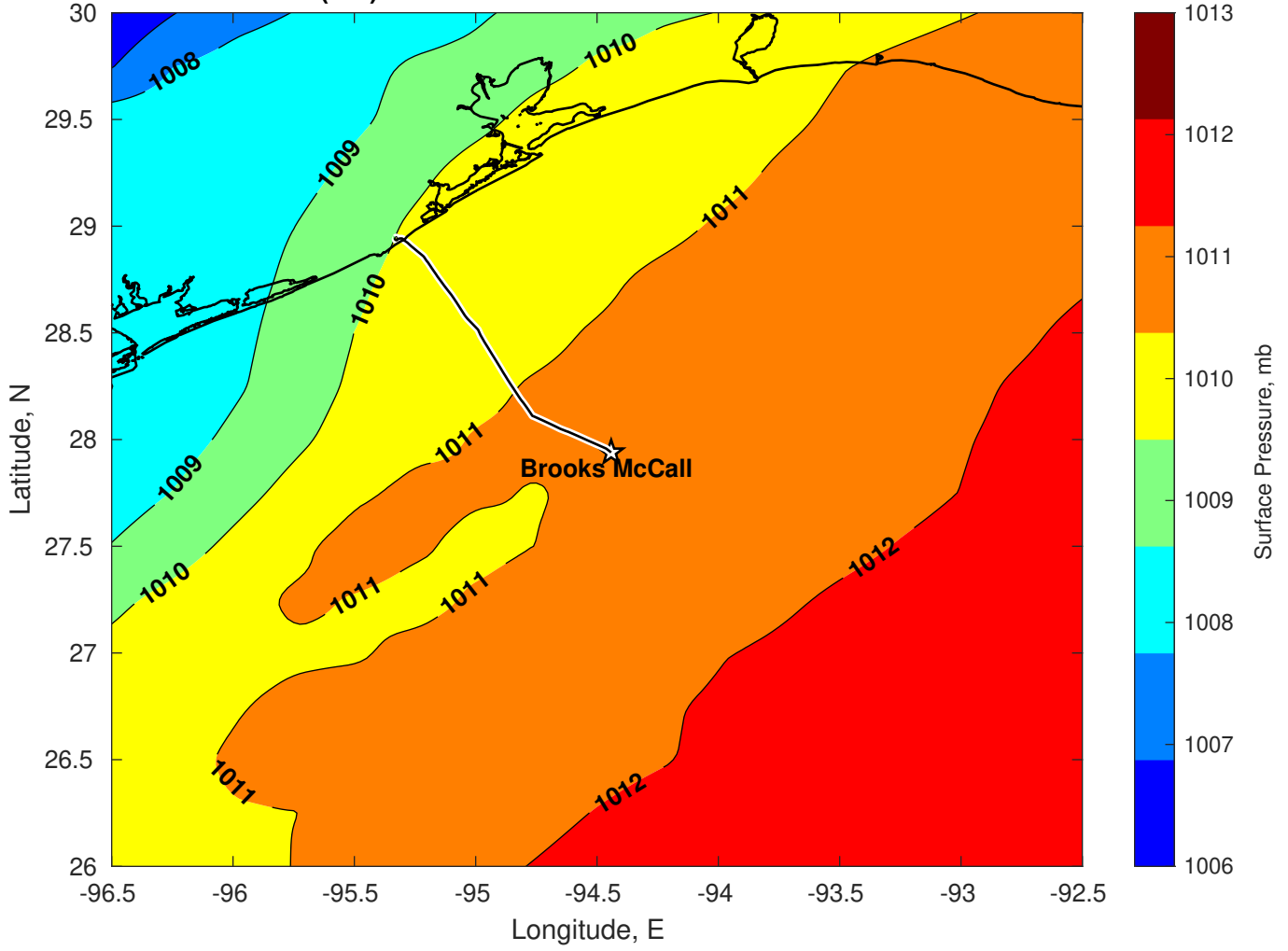
Surface Pressure (mb) for Brooks McCall at 13-Mar-2025 00:00:00
