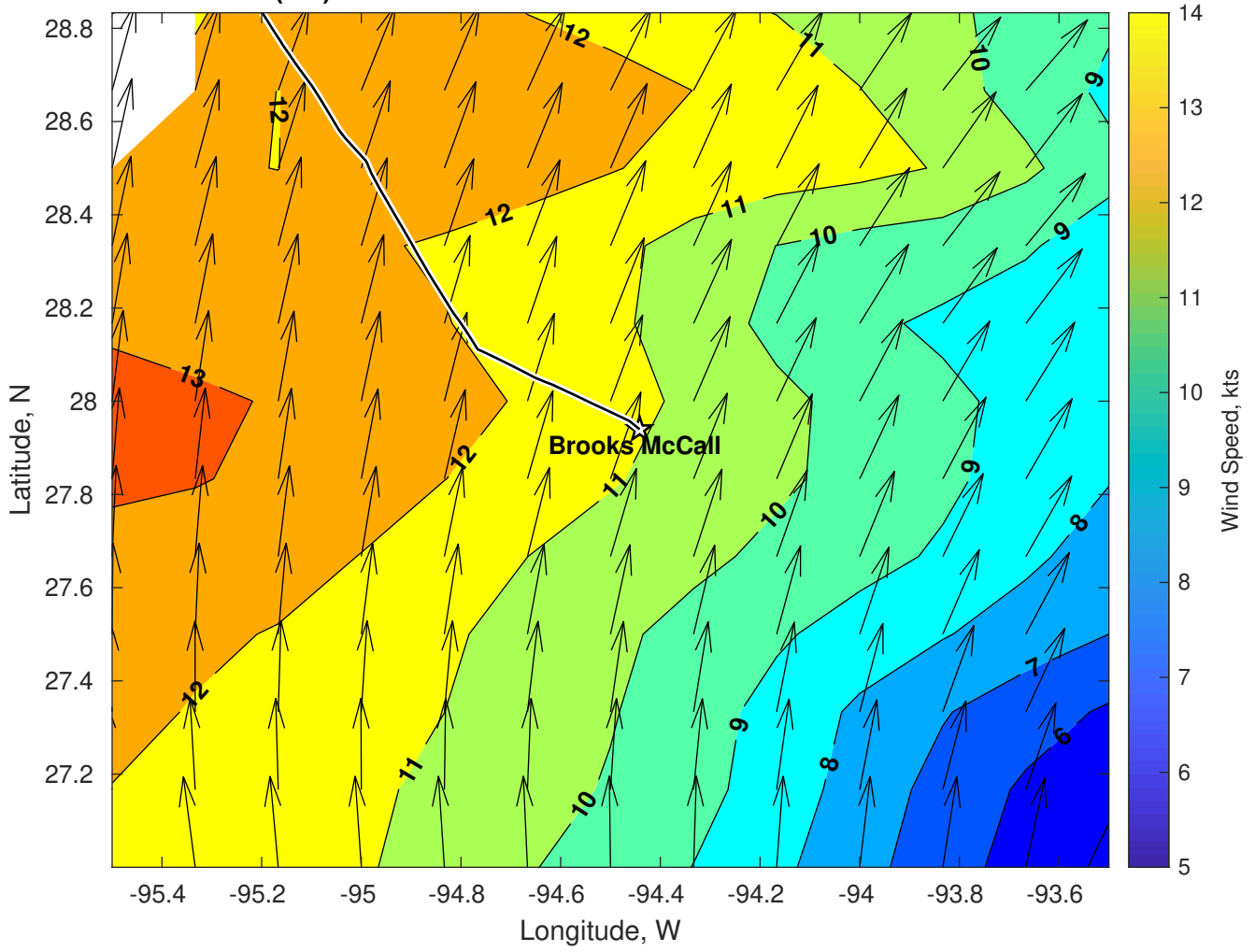
Winds (kts) for Brooks McCall at 11-Mar-2025 09:00:00
