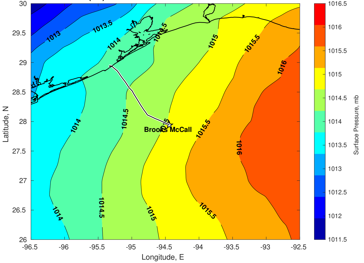
Surface Pressure (mb) for Brooks McCall at 12-Mar-2025 00:00:00
