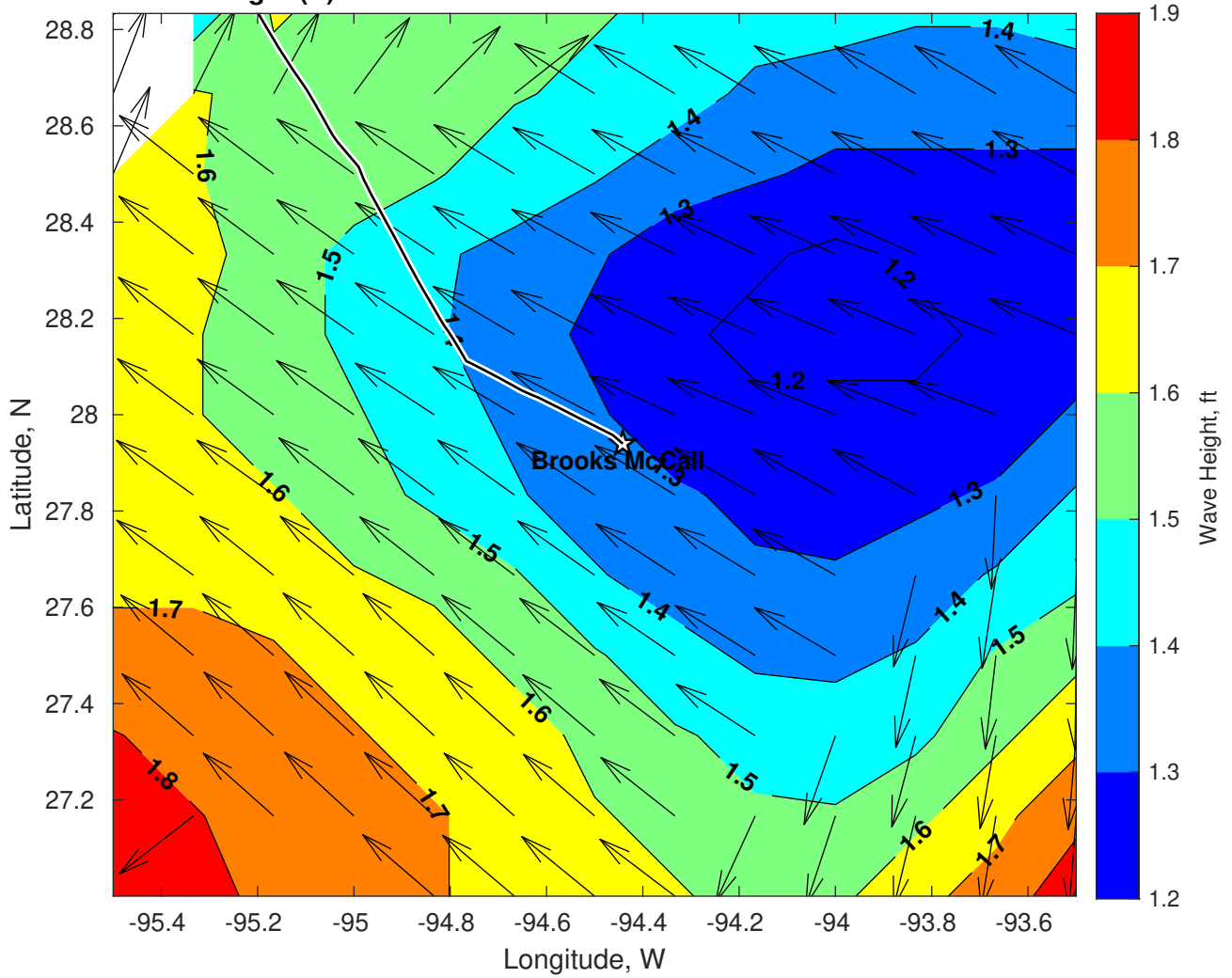
Wave Height (ft) for Brooks McCall at 11-Mar-2025 09:00:00
