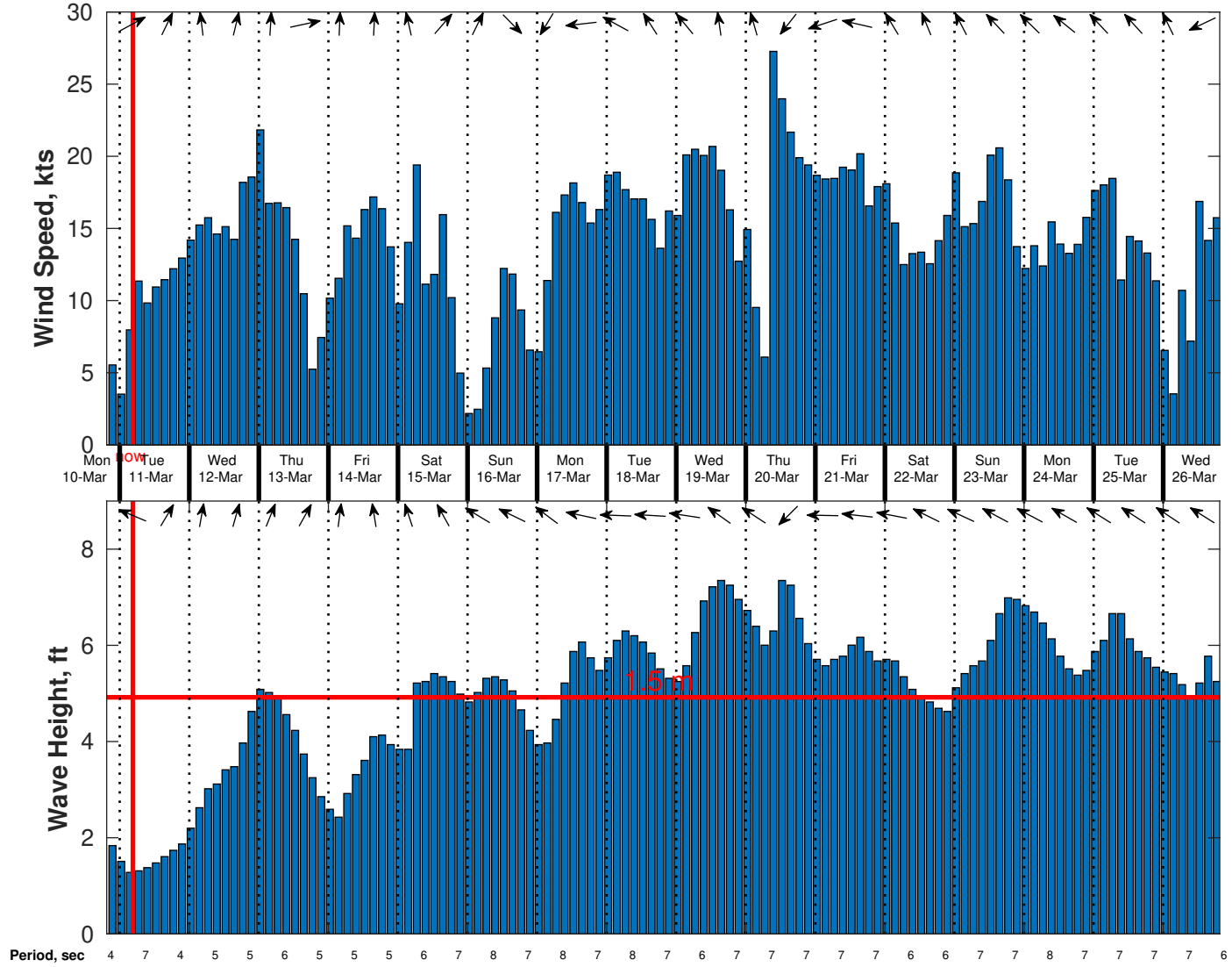
Wind & Wave Forecast for Brooks McCall from 10-Mar-2025 20:00:00 to 26-Mar-2025 20:00:00
