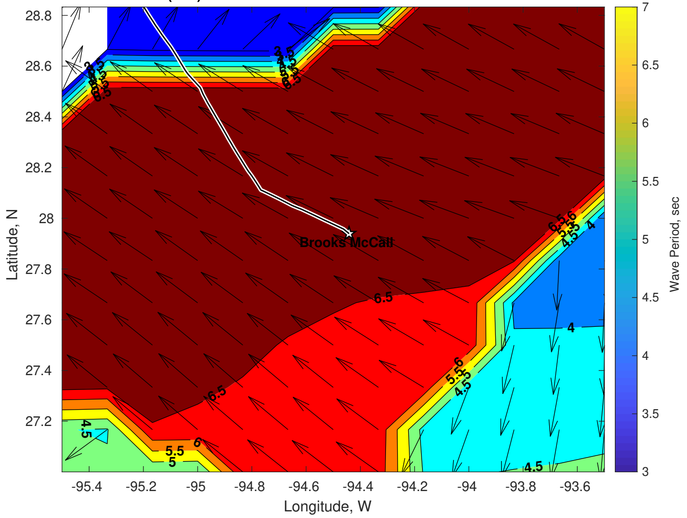
Wave Period (sec) for Brooks McCall at 11-Mar-2025 09:00:00
