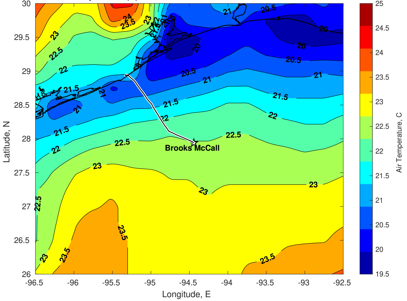
Air Temperature (C) for Brooks McCall at 11-Mar-2025
