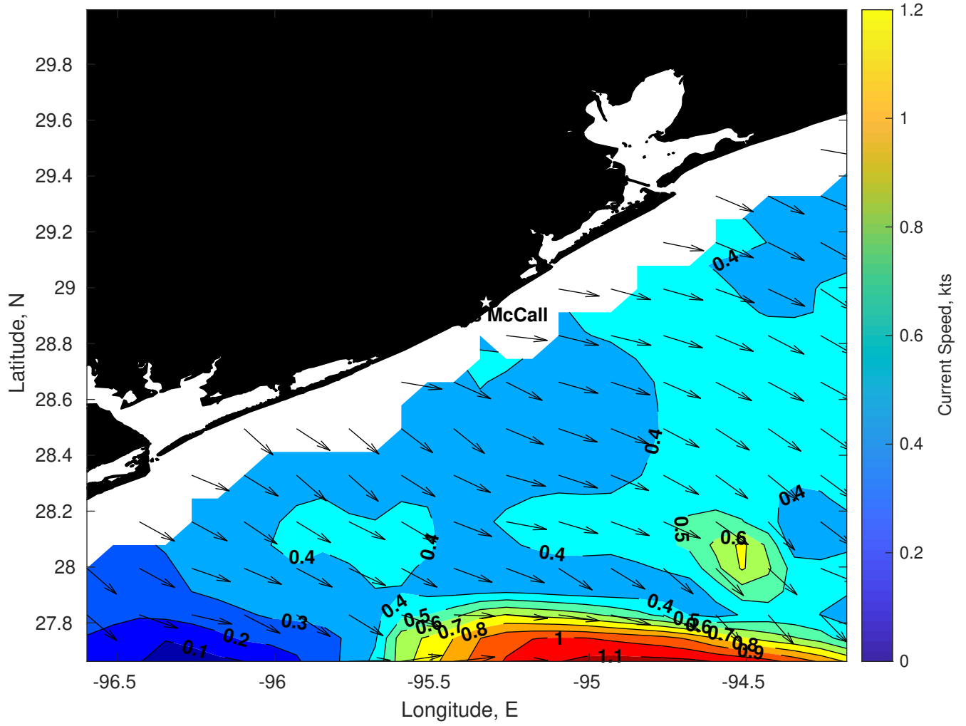
Surface Currents for Brooks McCall at 10-Mar-2025 00:00:00
