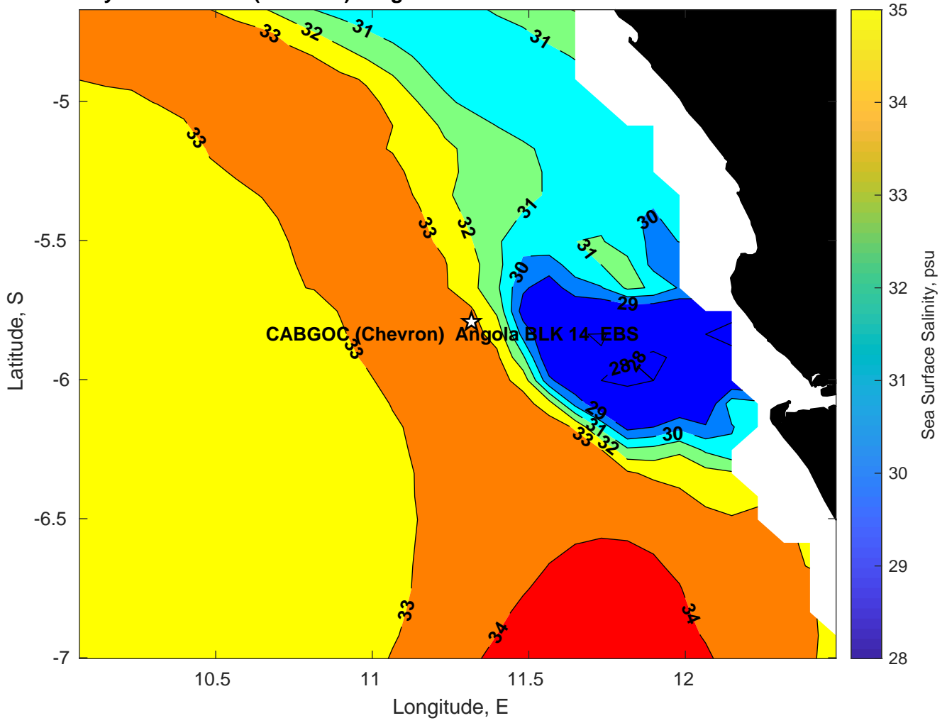
Surface Salinity for CABGOC (Chevron) Angola BLK 14 EBS at 10-Mar-2025 00:00:00
