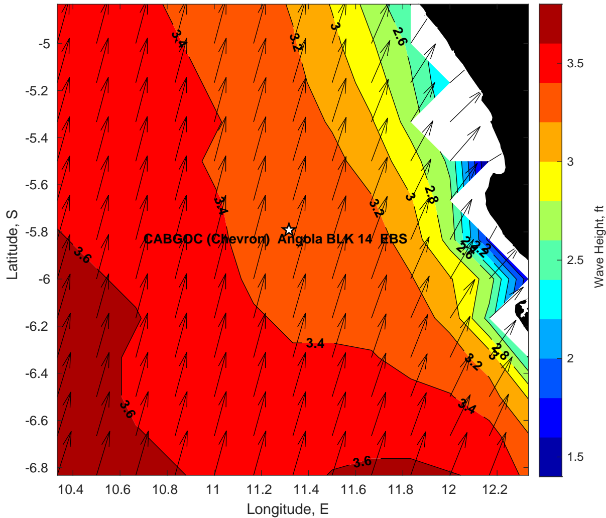
Wave Height (ft) for CABGOC (Chevron) Angola BLK 14 EBS at 11-Mar-2025 09:00:00
