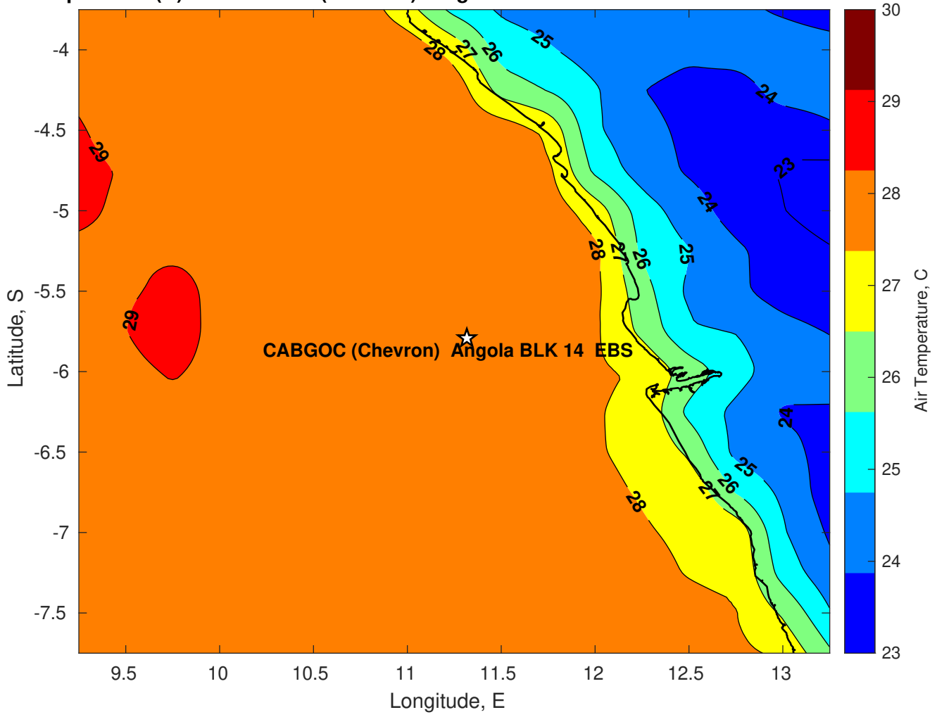
Air Temperature (C) for CABGOC (Chevron) Angola BLK 14 EBS at 11-Mar-2025
