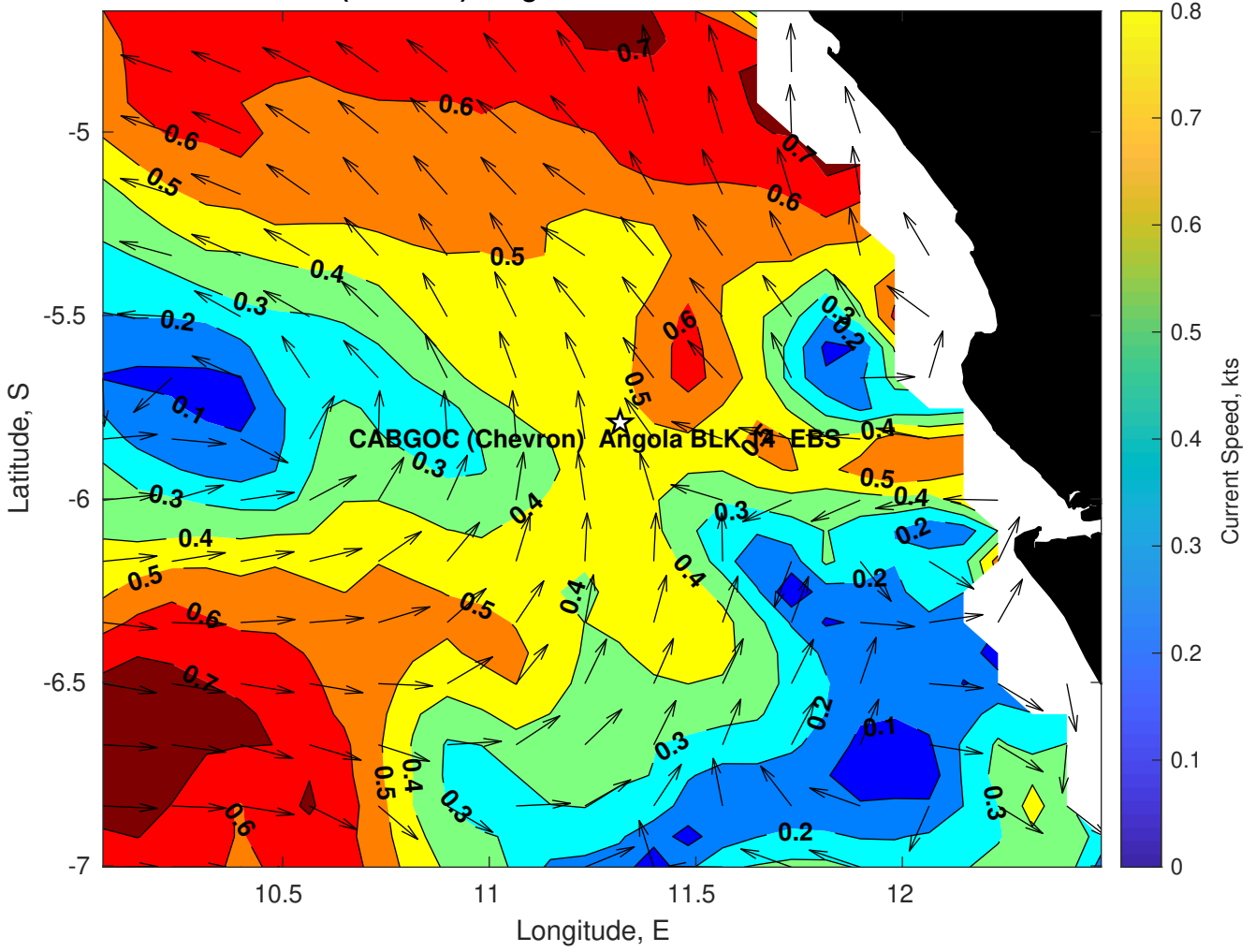
Surface Currents for CABGOC (Chevron) Angola BLK 14 EBS at 10-Mar-2025 00:00:00
