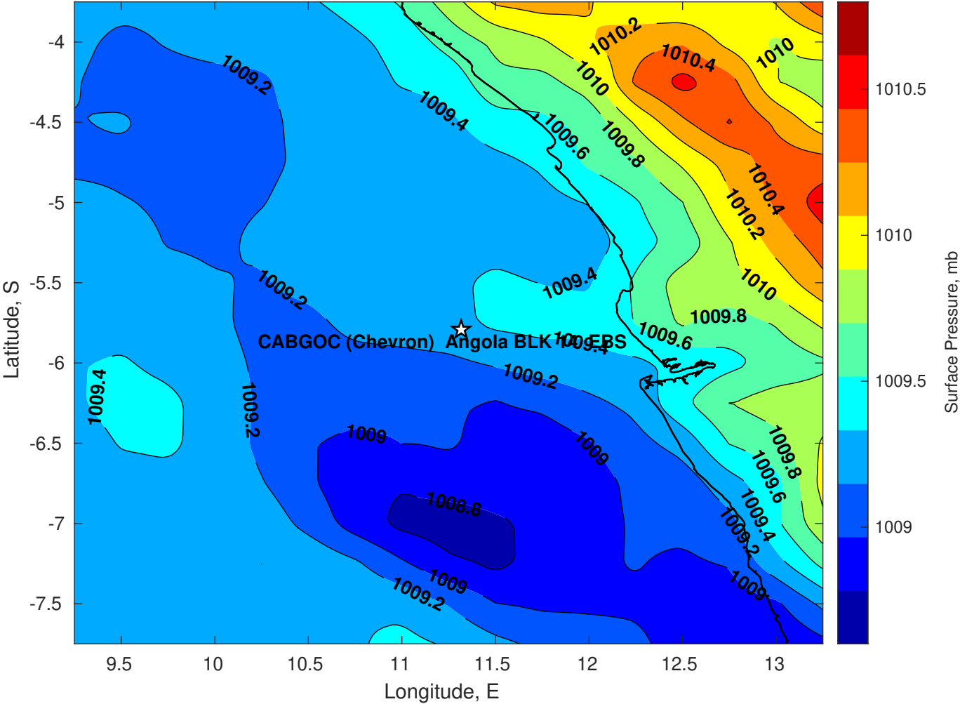
Surface Pressure (mb) for CABGOC (Chevron) Angola BLK 14 EBS at 13-Mar-2025 00:00:00
