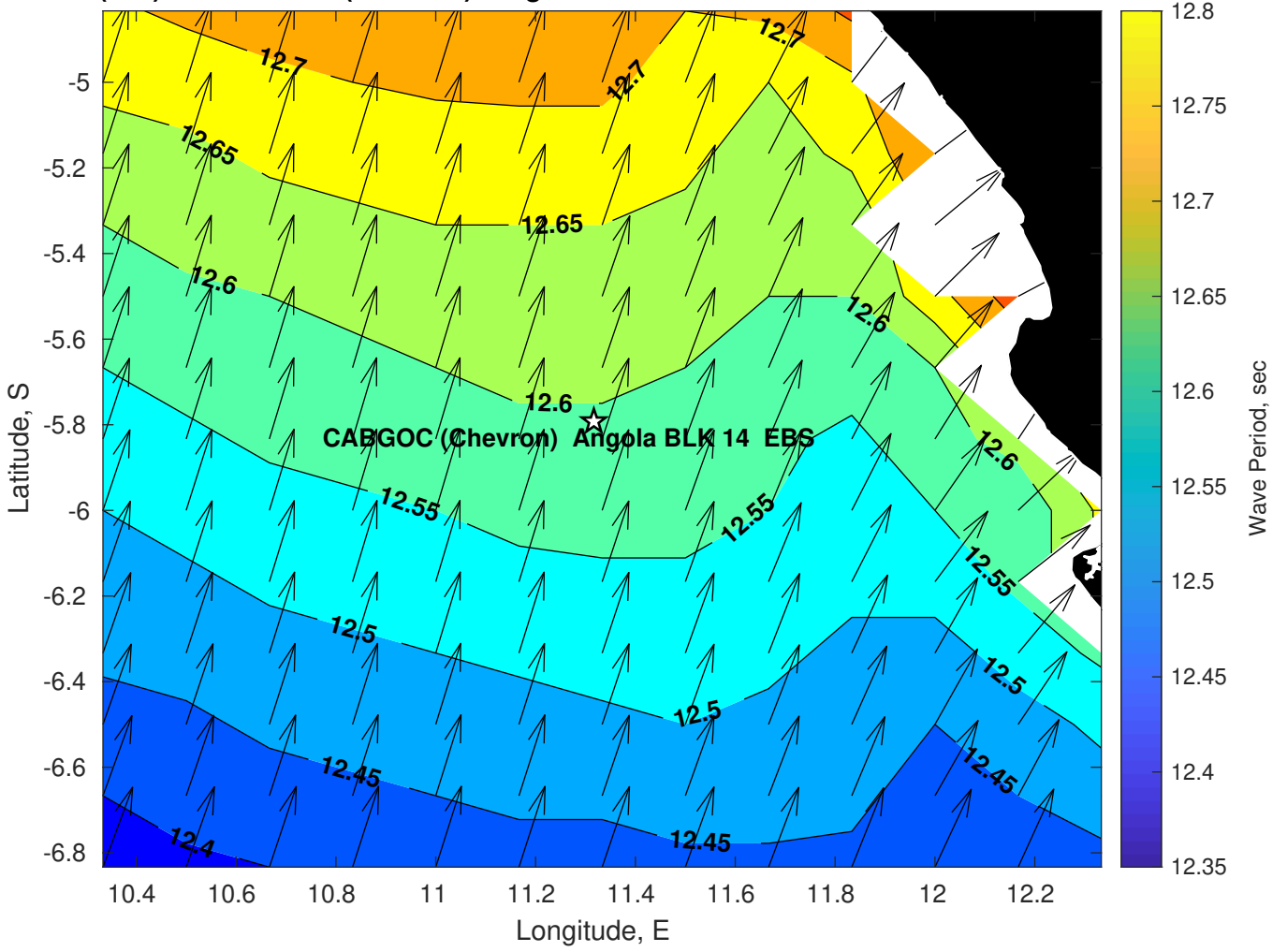
Wave Period (sec) for CABGOC (Chevron) Angola BLK 14 EBS at 11-Mar-2025 09:00:00
