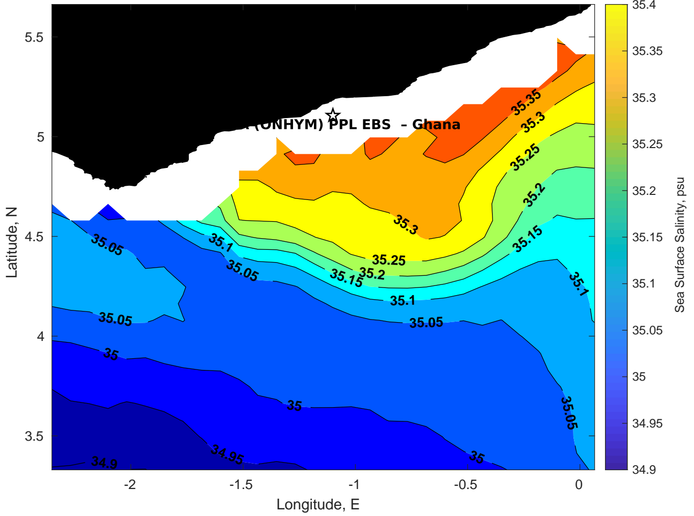
Surface Salinity for CSA (ONHYM) PPL EBS - Ghana at 10-Mar-2025 00:00:00
