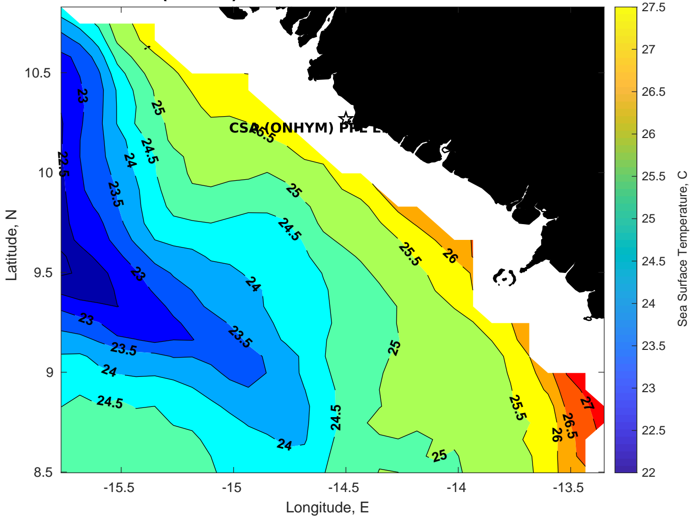
SST for CSA (ONHYM) PPL EBS - Guinea at 10-Mar-2025 00:00:00
