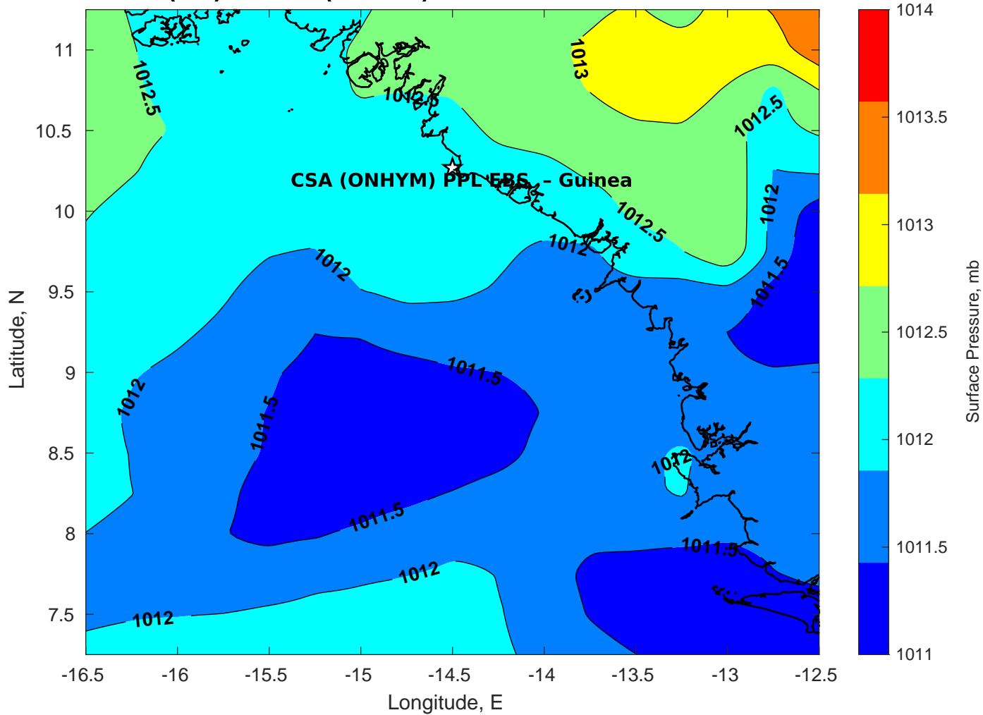
Surface Pressure (mb) for CSA (ONHYM) PPL EBS - Guinea at 13-Mar-2025 00:00:00
