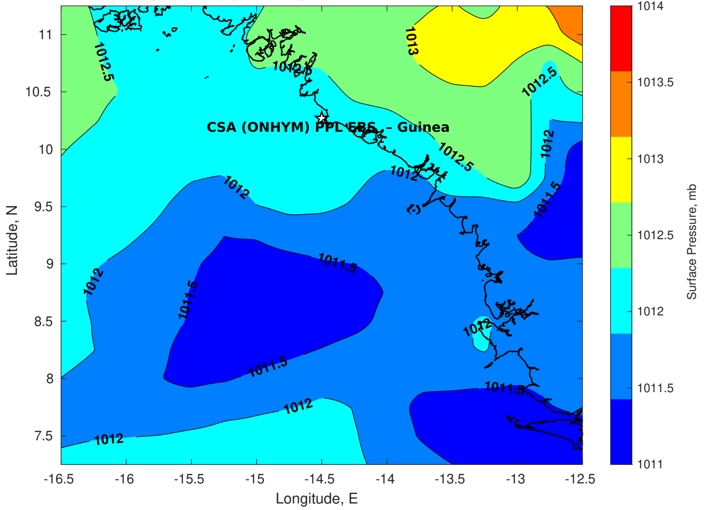
Surface Pressure (mb) for CSA (ONHYM) PPL EBS - Guinea at 13-Mar-2025 00:00:00
