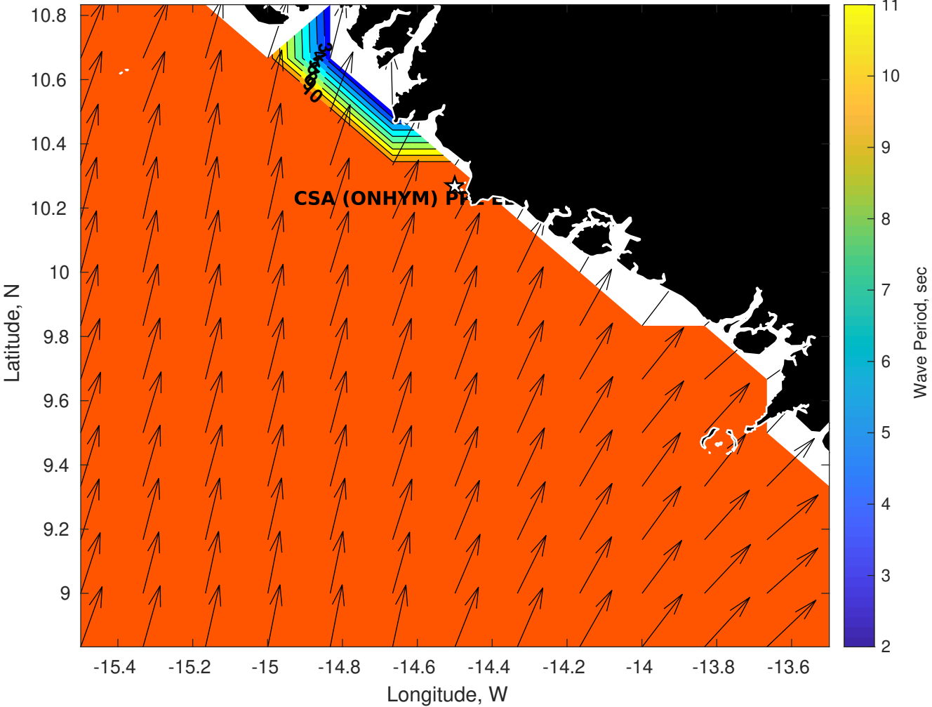
Wave Period (sec) for CSA (ONHYM) PPL EBS - Guinea at 11-Mar-2025 09:00:00
