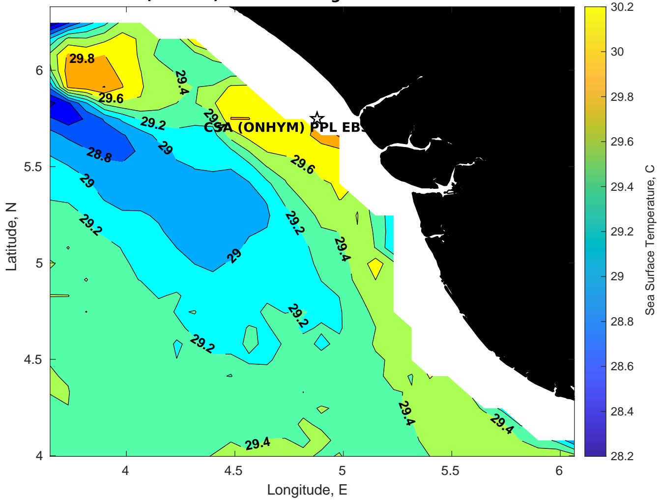
SST for CSA (ONHYM) PPL EBS - Nigeria at 10-Mar-2025 00:00:00
