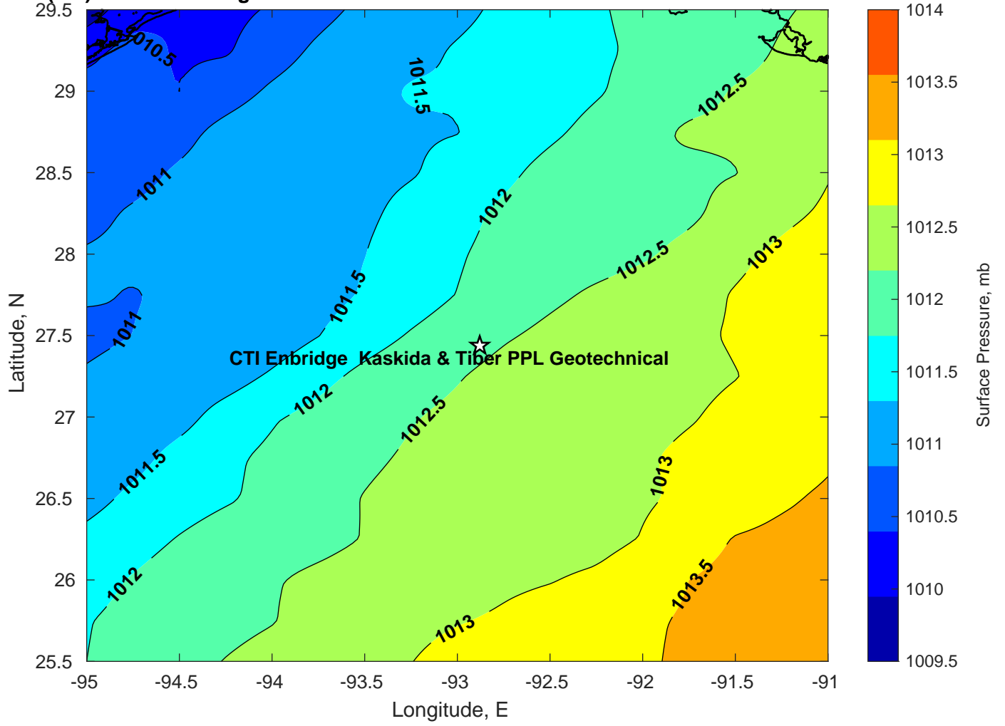
Surface Pressure (mb) for CTI Enbridge Kaskida & Tiber PPL Geotechnical at 13-Mar-2025 00:00:00
