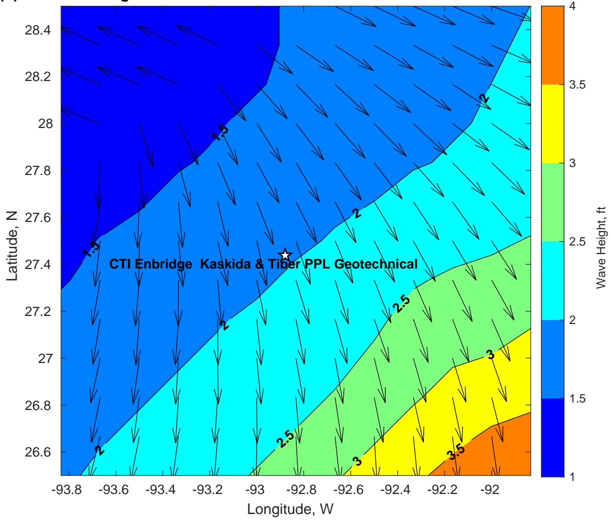
Wave Height (ft) for CTI Enbridge Kaskida & Tiber PPL Geotechnical at 11-Mar-2025 09:00:00
