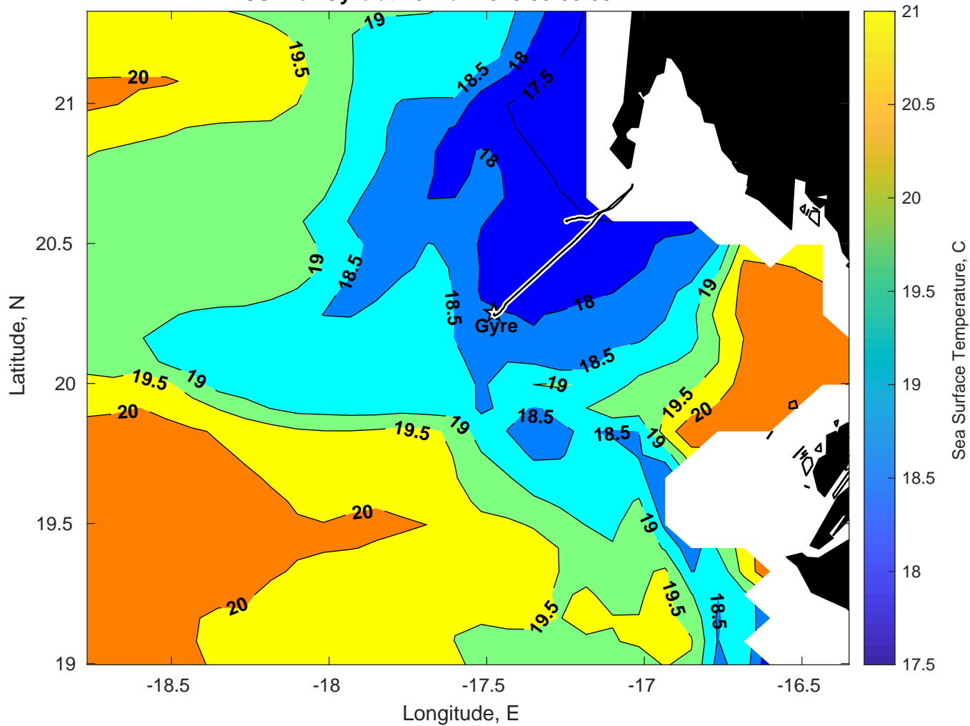
SST for Gyre at 10-Mar-2025 00:00:00
