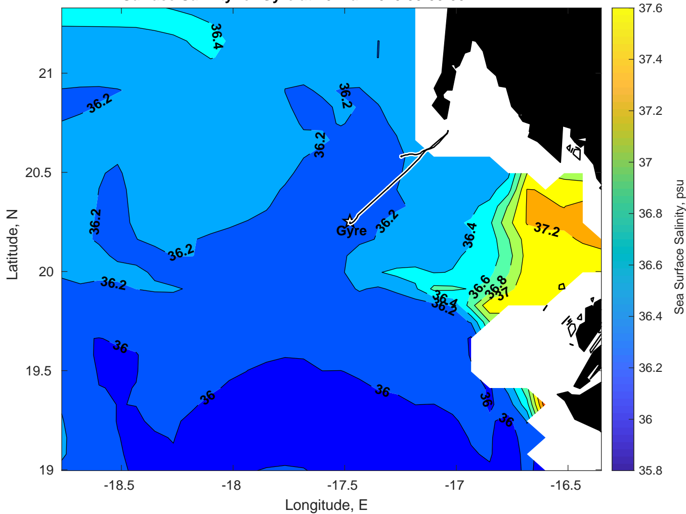
Surface Salinity for Gyre at 10-Mar-2025 00:00:00
