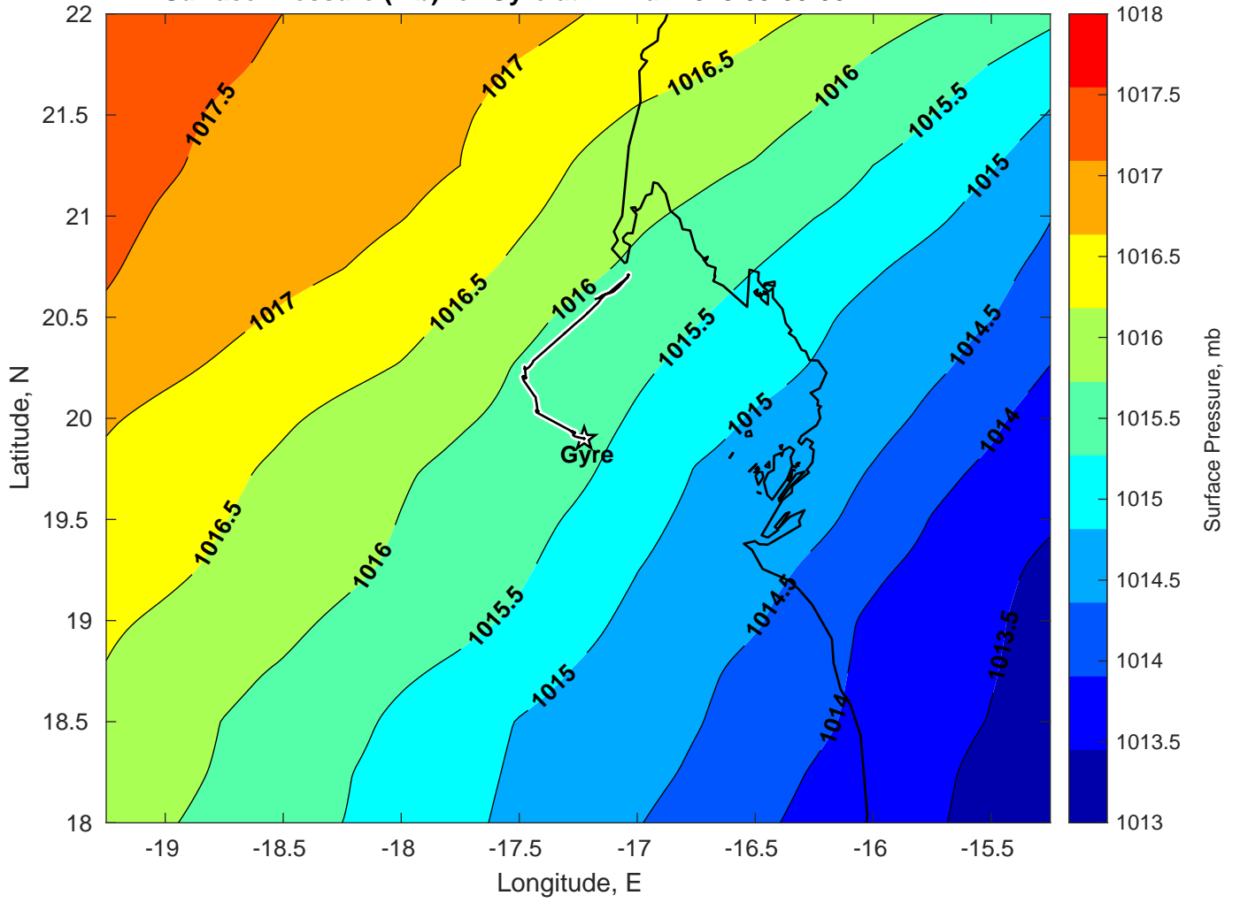
Surface Pressure (mb) for Gyre at 11-Mar-2025 00:00:00
