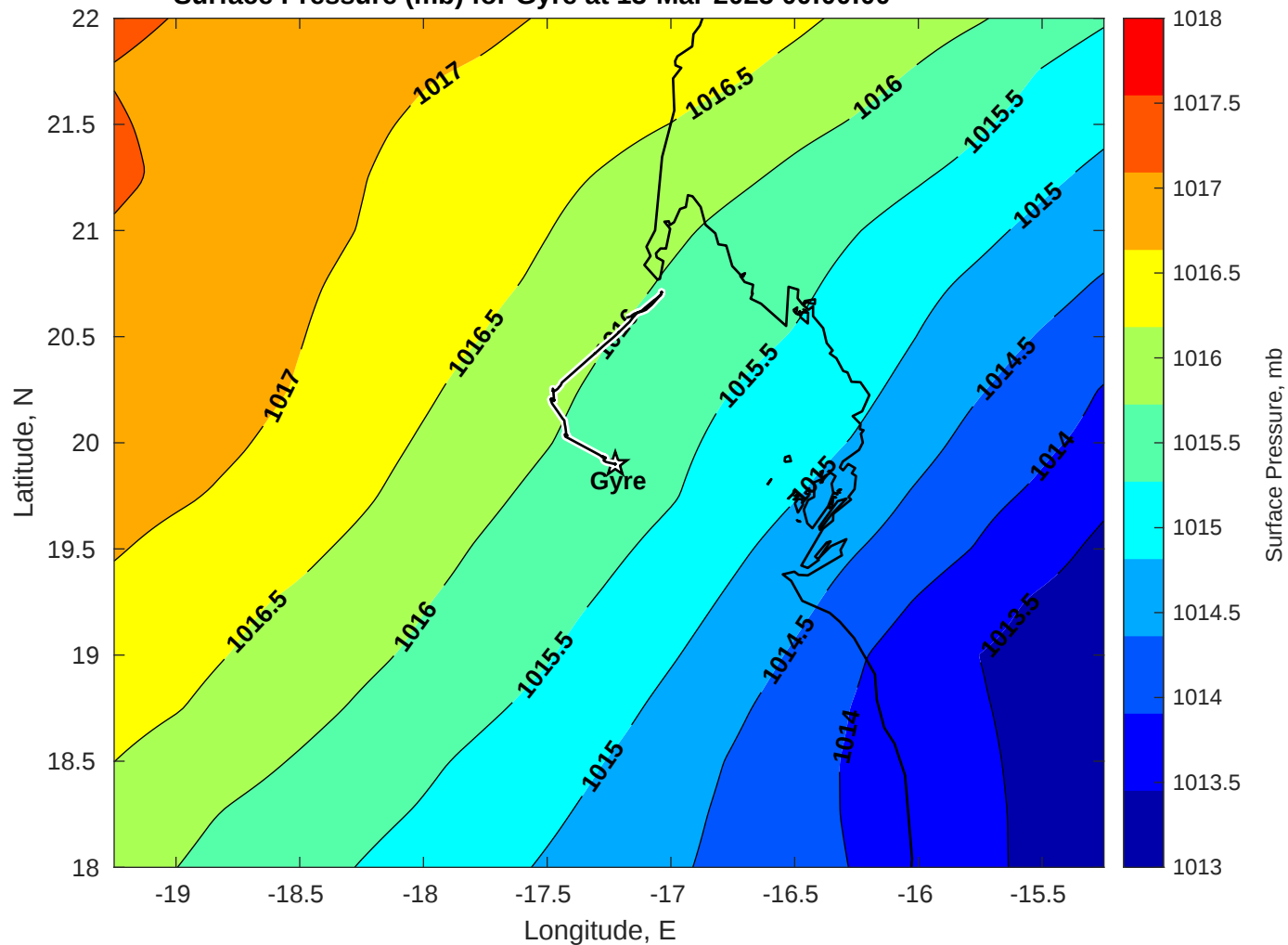
Surface Pressure (mb) for Gyre at 13-Mar-2025 00:00:00
