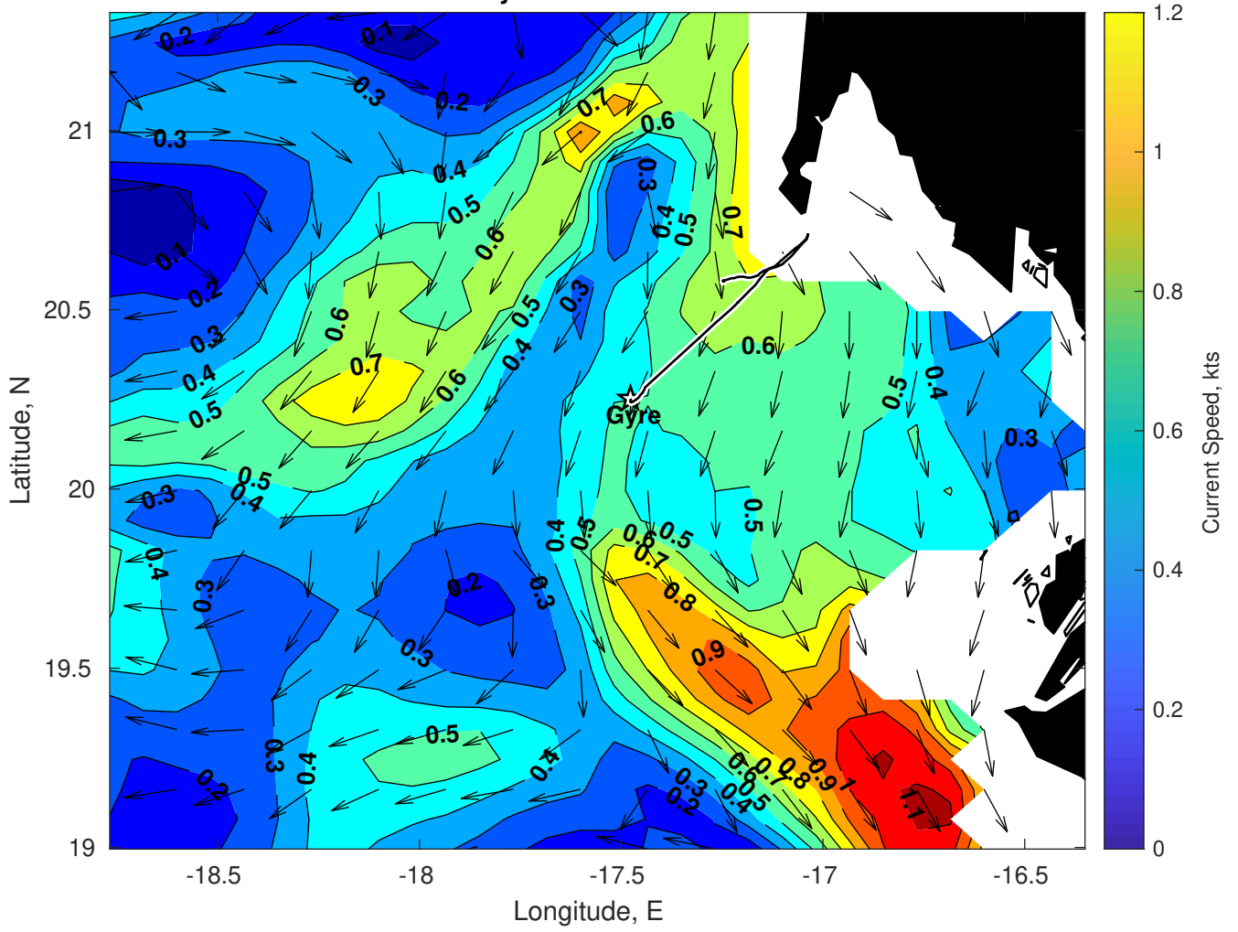
Surface Currents for Gyre at 10-Mar-2025 00:00:00
