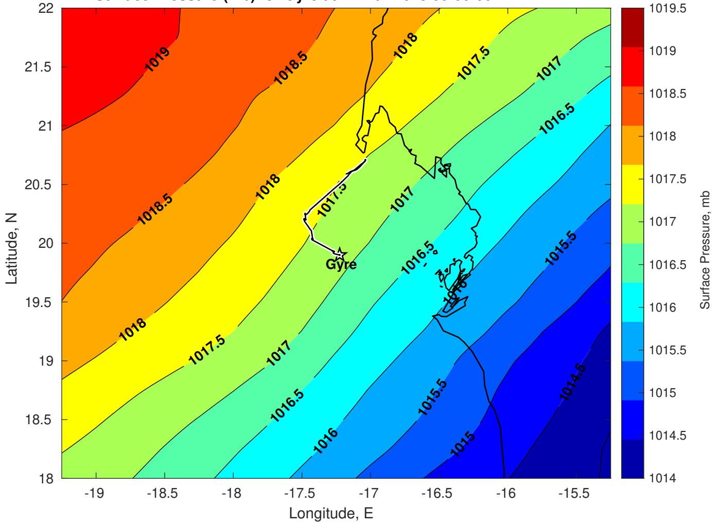
Surface Pressure (mb) for Gyre at 12-Mar-2025 00:00:00
