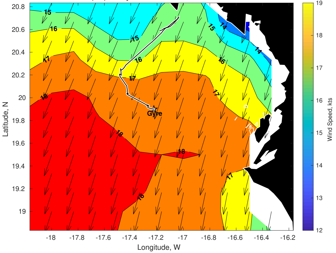
Winds (kts) for Gyre at 11-Mar-2025 09:00:00
