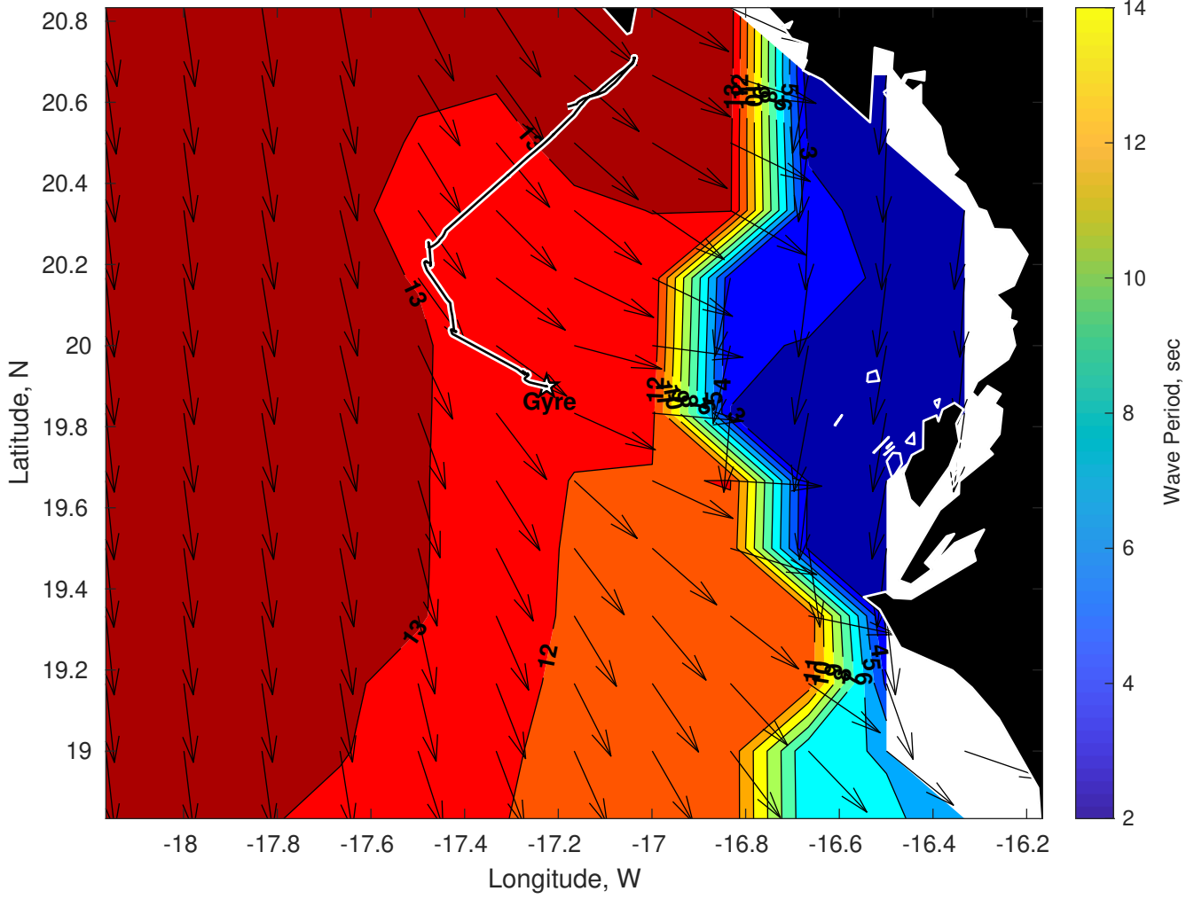
Wave Period (sec) for Gyre at 11-Mar-2025 09:00:00
