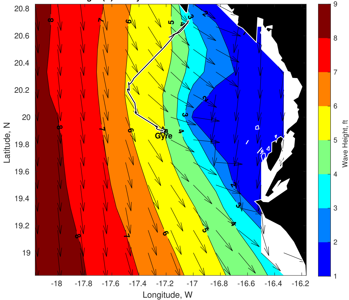
Wave Height (ft) for Gyre at 11-Mar-2025 09:00:00
