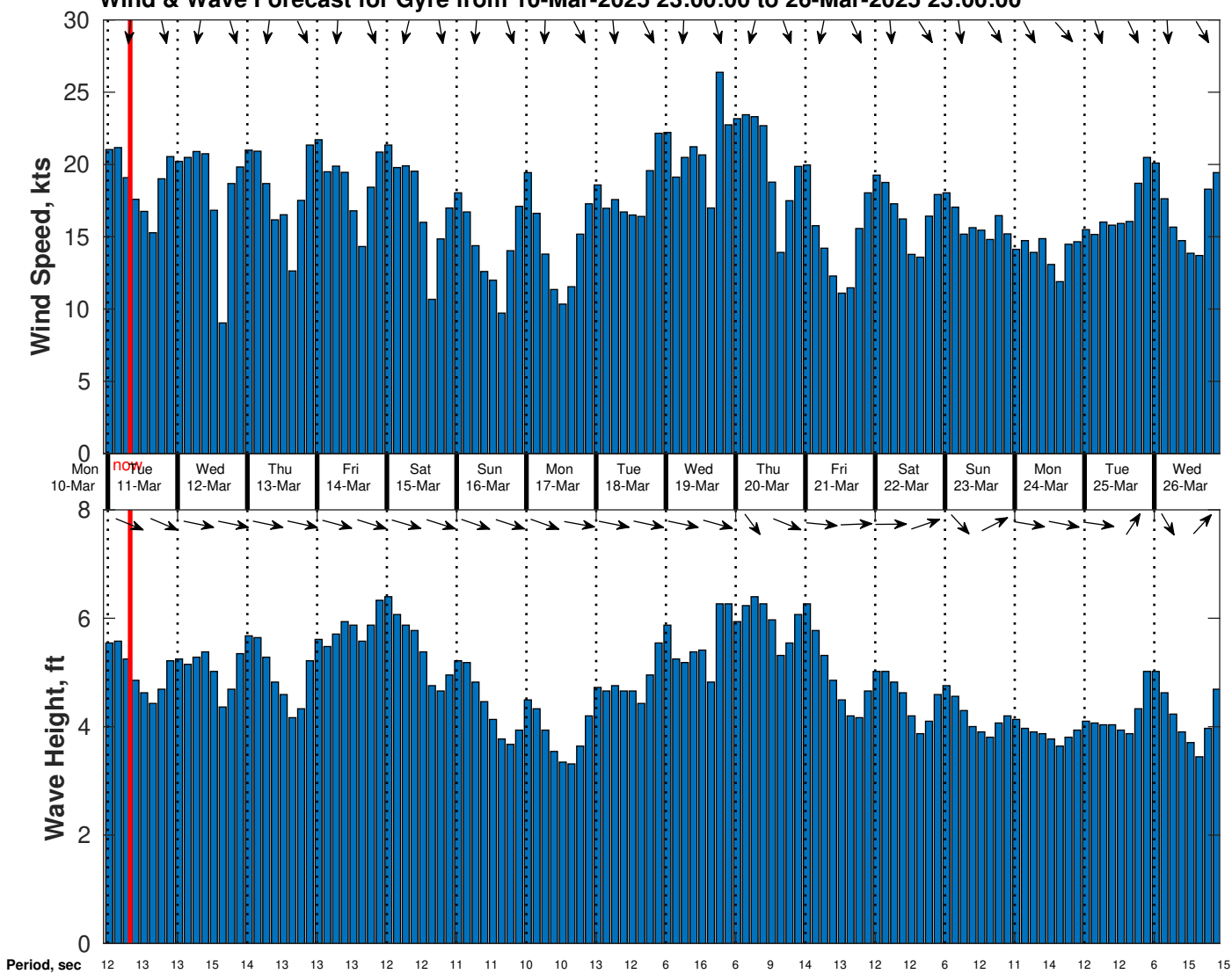
Wind & Wave Forecast for Gyre from 10-Mar-2025 23:00:00 to 26-Mar-2025 23:00:00
